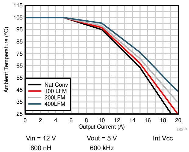
Figure 6-6. Safe Operating Area, V OUT = 5 V
