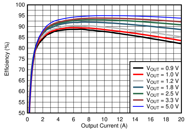
Figure 6-4. Efficiency vs Output Current, 12 V IN , 800 kHz, FCCM, VCC = EXT 3.3 V
