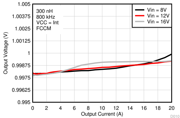
8-8. Output Voltage vs Output Current
