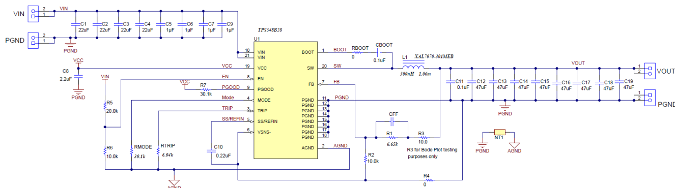
8-1. TPS548B28 Application Circuit Diagram
