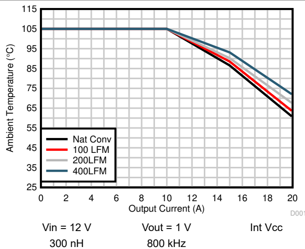
Figure 6-5. Safe Operating Area, V OUT = 1.0 V
