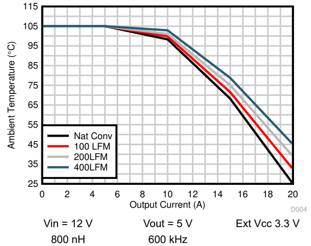
Figure 6-8. Safe Operating Area, V_{OUT} = 5\text{ V}
