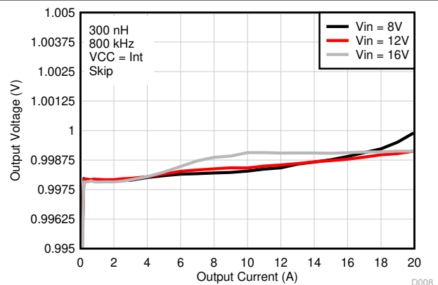
8-7. Output Voltage vs Output Current
