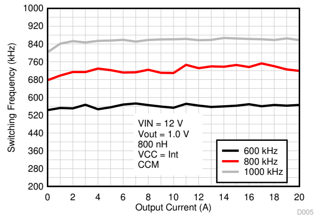
8-5. Switching Frequency vs Output Current
