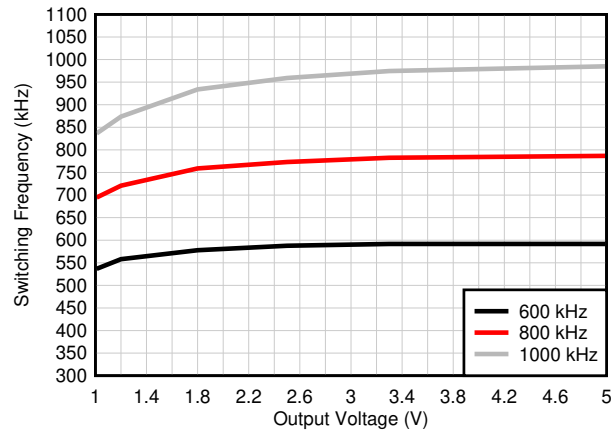
Figure 6-9. Switching Frequency vs Output Voltage
