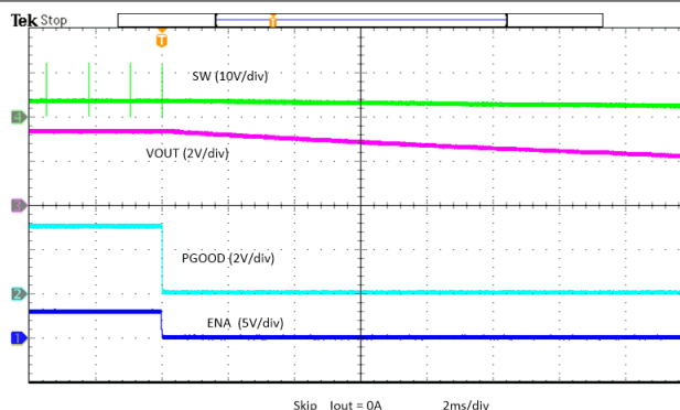
8-17. Enable Power Down, Skip
