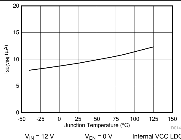
Figure 6-11. I_{SD(VIN)} vs Junction Temperature
