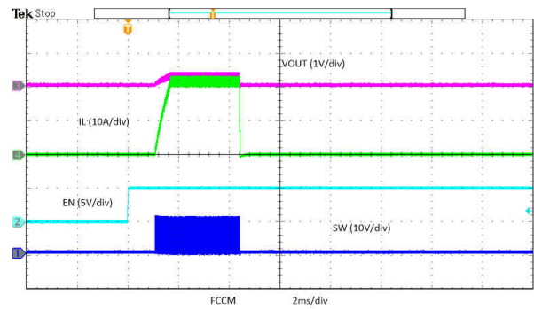
8-29. Enabled into Overcurrent
