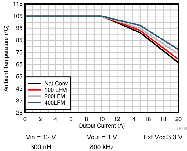
Figure 6-7. Safe Operating Area, V_{OUT} = 1\text{ V}
