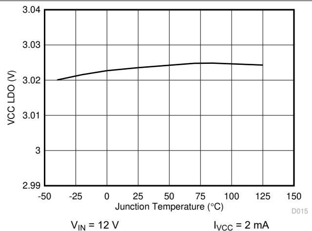
Figure 6-12. VCC LDO vs Junction Temperature
