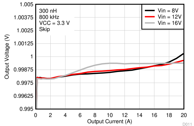
8-9. Output Voltage vs Output Current, VCC = 3.3-V External Bias
