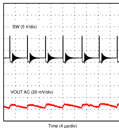
Time (4 \mu s/div) V_{IN} = 12 V I_{LOAD} = 0.1 A MODE = DCM
