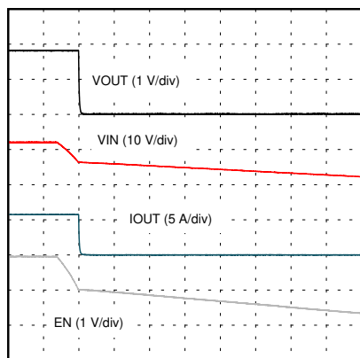
Time (4 ms/div) R_{LOAD} = 0.3 \Omega 図 7-20. V_{IN} Shutdown
