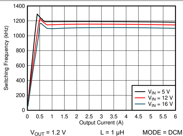
5-18. 1100 kHz Switching Frequency vs Load Current – DCM
