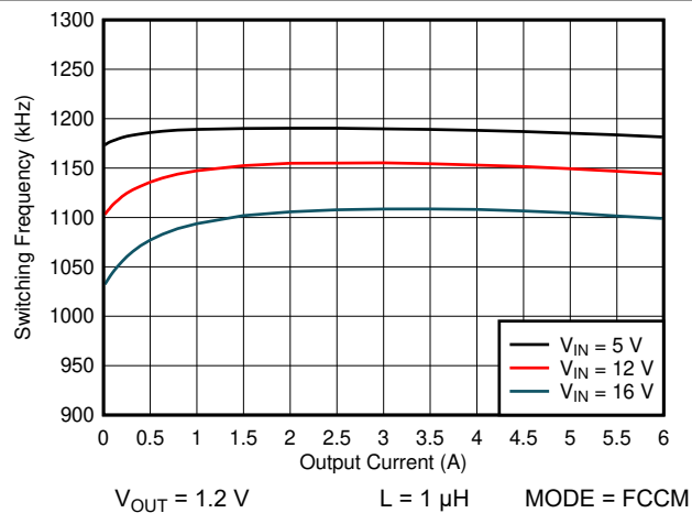
5-16. 1100 kHz Switching Frequency vs Load Current
