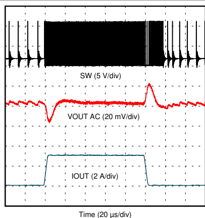
Time (20 \mu s/div) V_{IN} = 12 V 0.1 A to 3.1 A step 1 A/ \mu sec MODE = DCM
