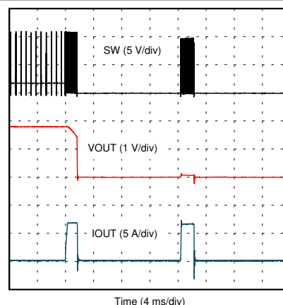
図 7-29. Overcurrent Response
