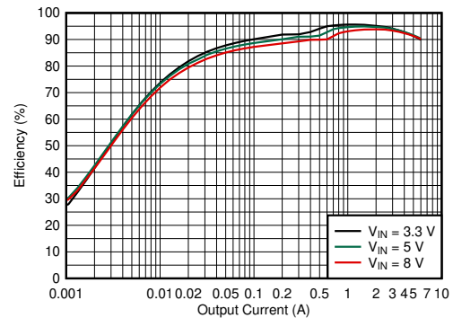
図 7-5. Efficiency – 1100 kHz, FFCM, External 3.3-V VCC, 0- \Omega R_{BOOT}
