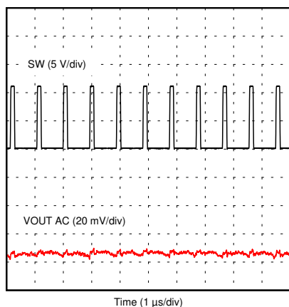
Time (1 \mu s/div) V_{IN} = 12 V I_{LOAD} = 0.1 A MODE = FCCM
