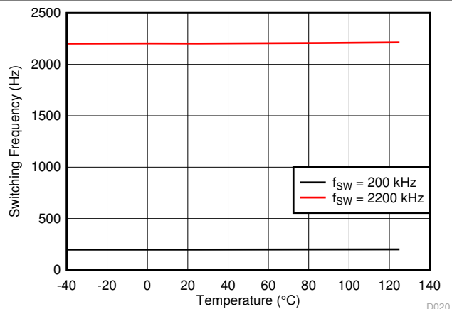
6-20. Switching Frequency vs Temperature
