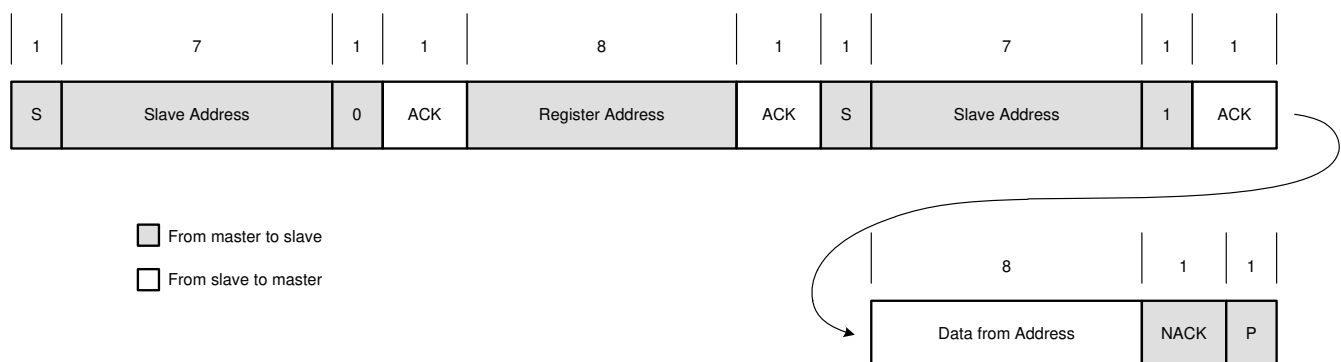
FIG 7-12. Single-byte Read
