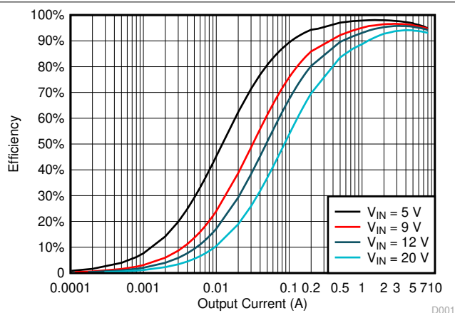
Figure 6-1. Efficiency vs Output Current, V_{OUT} = 5\text{ V} , FPWM
