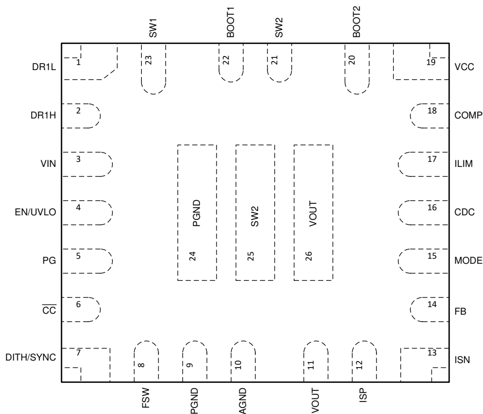
5-1. TPS552882 26-pin VQFN-HR Transparent Top View
