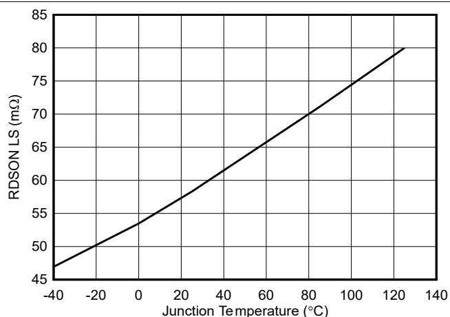
図 5-6. High-Side Rdson
