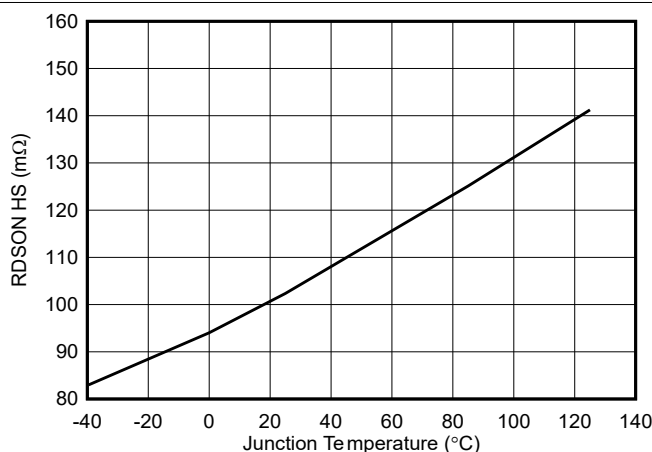
図 5-5. Low-Side Rdson
