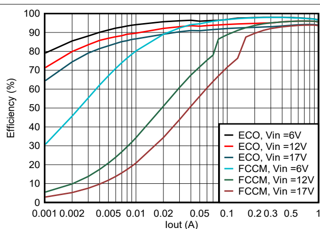
図 5-12. TPS56124x Efficiency at 5 Vout With 3.3uH Inductor
