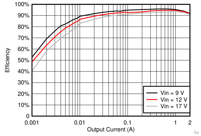
7-14. V_{OUT} = 5\text{-V} Efficiency, L = 4.7\text{ }\mu\text{H}
