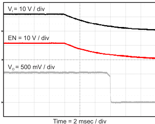
図 8-14. Tps562200 Shut Down Relative to V_I
