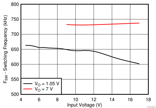
Figure 6-17. Switching Frequency vs Input Voltage I_{OUT} = 1\text{ A}
