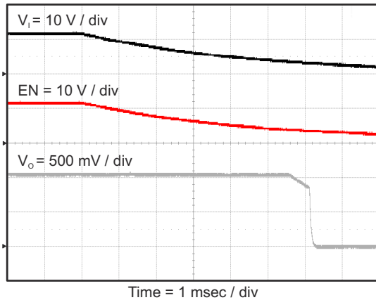
FIG 8-29. Tps563200 Shut Down Relative to V_i
