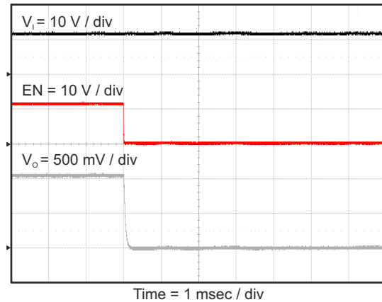
FIG 8-30. Tps563200 Shutdown Relative to En
