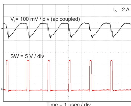
Figure 8-7. Tps562200 Input Voltage Ripple
