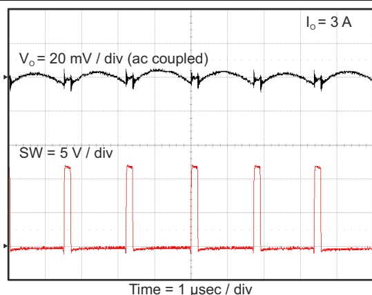
8-25. Tps563200 Output Voltage Ripple
