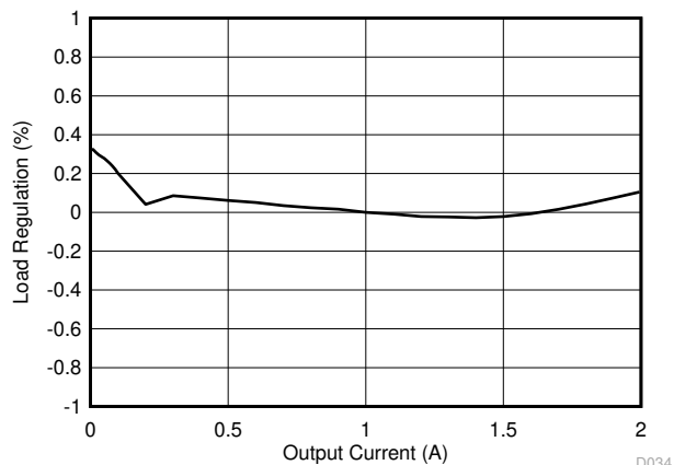
Figure 8-5. Tps562200 Load Regulation, V_I = 12\text{ V}
