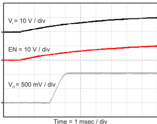
8-27. Tps563200 Start-up Relative to V_i
