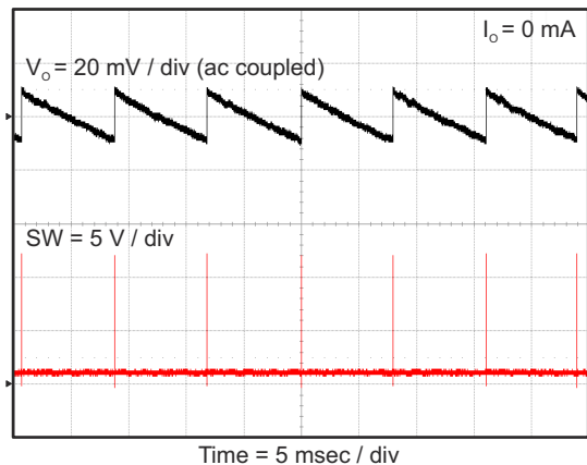
8-23. Tps563200 Output Voltage Ripple
