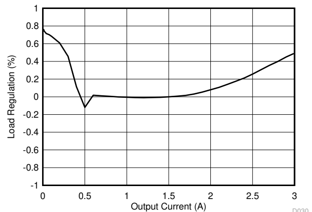
图 8-20. Tps563200 Load Regulation, V_I = 12\text{ V}
