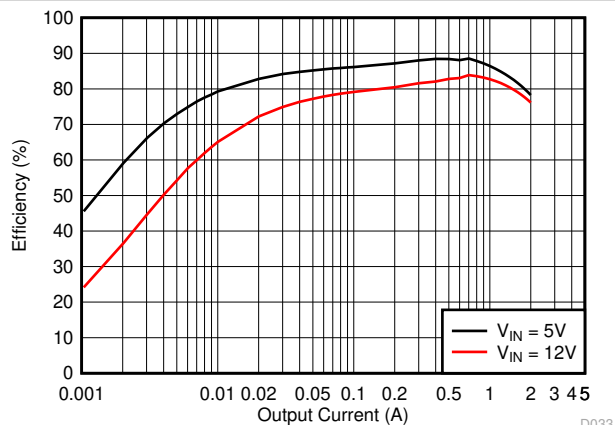
Figure 8-3. Tps562200 Light Load Efficiency
