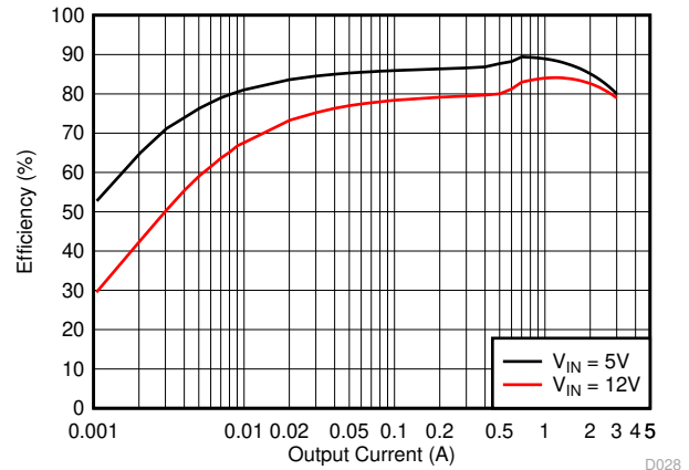
图 8-18. Tps563200 Light Load Efficiency
