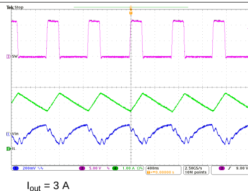
Figure 21. Input Voltage Ripple
