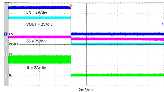
图 8-11. Shutdown Through EN, I_{OUT} = 3\text{ A}
