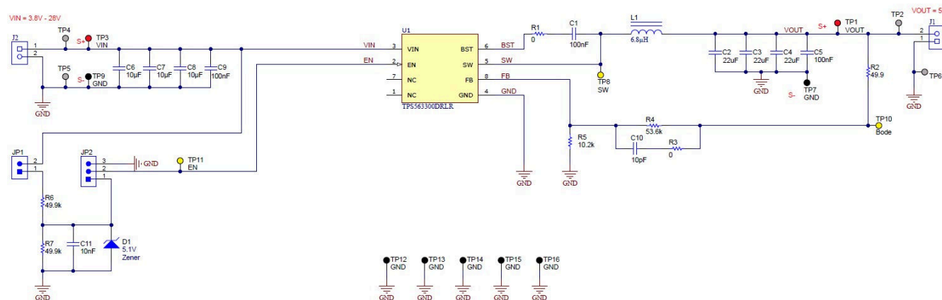
8-1. TPS563300 5-V Output, 3-A Reference Design
