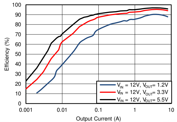
Fig 6-12. Efficiency, Mode = DCM, F_{SW} = 400kHz
