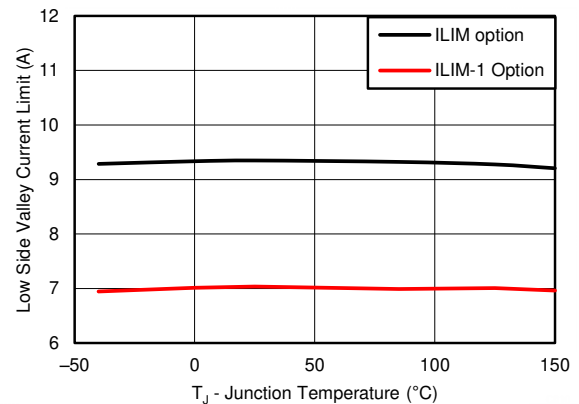
Fig 6-10. Valley Current Limit vs Temperature
