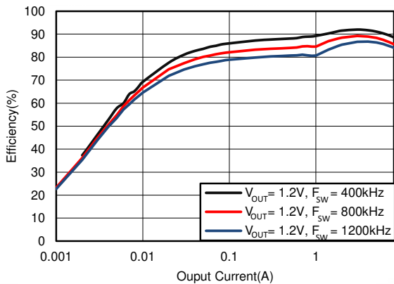
Fig 6-11. Efficiency with Internal VREG5 = 4.7 V, V_{IN} = 12 V
