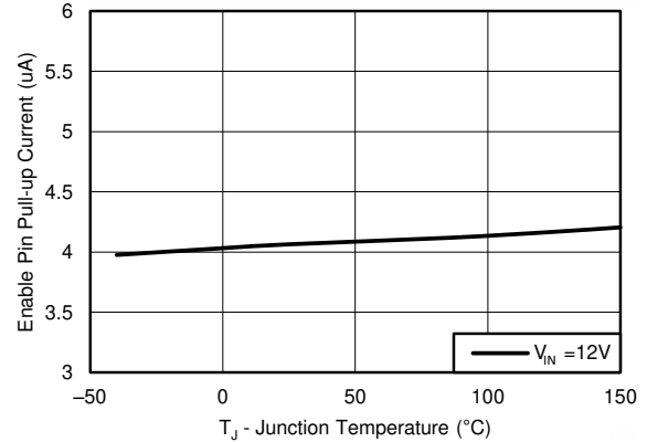
Fig 6-8. Enable Pull-Up Current, V_{EN} = 1.3V
