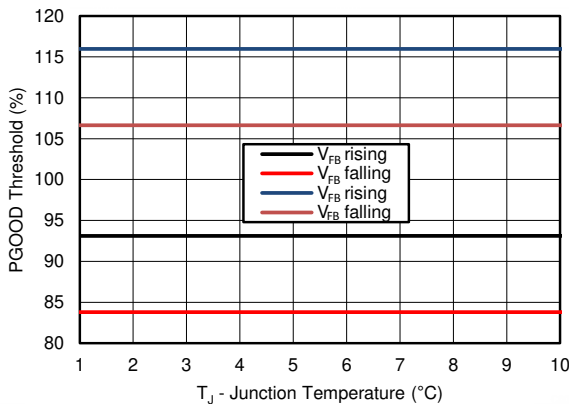
Fig 6-9. PGOOD Threshold vs Temperature
