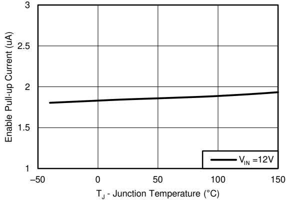
Fig 6-7. Enable Pull-Up Current, V_{EN} = 1.0V
