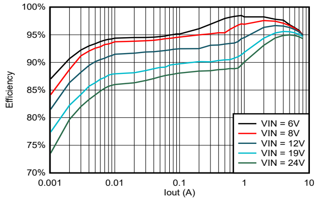
図 5-17. TPS56837 Efficiency, V_{out} = 5V , F_{sw} = 500kHz
