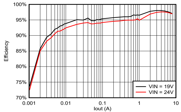
図 5-20. TPS56837 Efficiency, V_{out} = 12V , F_{sw} = 500kHz
