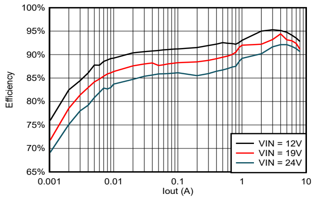
図 5-19. TPS56837 Efficiency, V_{out} = 5V , F_{sw} = 1200kHz
