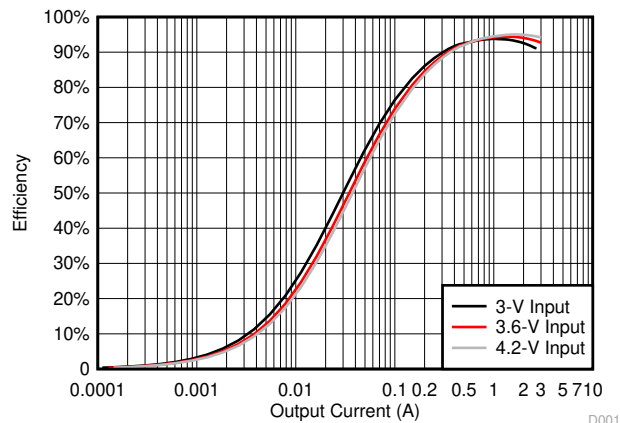
Figure 6-1. Efficiency vs Output Current, V_{OUT} = 9\text{ V} , FPWM
