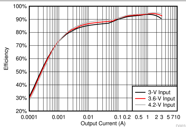
Figure 6-3. Efficiency vs Output Current, V_{OUT} = 9\text{ V} , PFM
