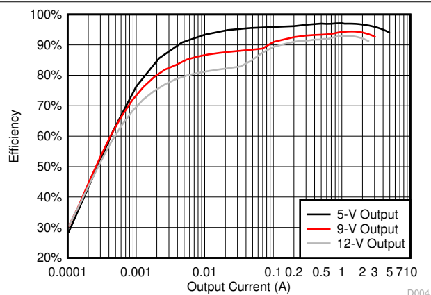
Figure 6-4. Efficiency vs Output Current, V_{IN} = 3.6\text{ V} , PFM
