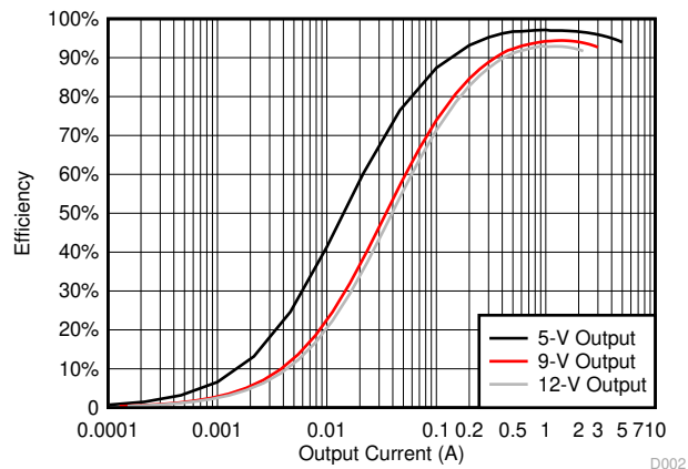
Figure 6-2. Efficiency vs Output Current, V_{IN} = 3.6\text{ V} , FPWM
