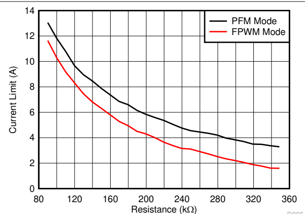
Figure 6-5. Current Limit vs Setting Resistance
