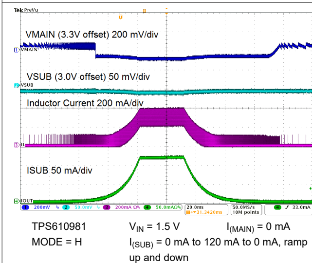
9-19. Load Regulation
