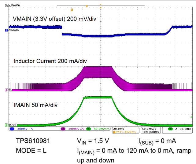
9-18. Load Regulation
