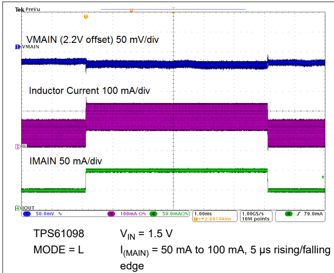
9-26. Load Transient Response
