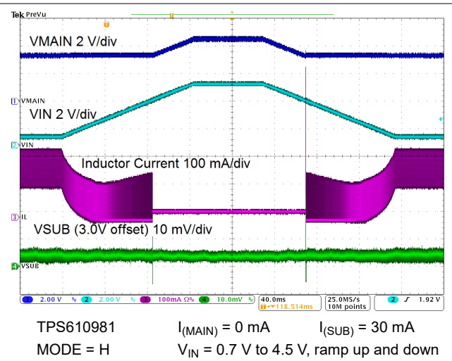
9-20. Line Regulation
