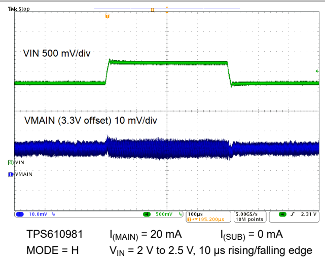
9-16. Line Transient Response
