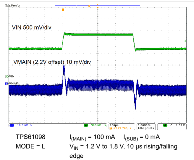
9-27. Line Transient Response
