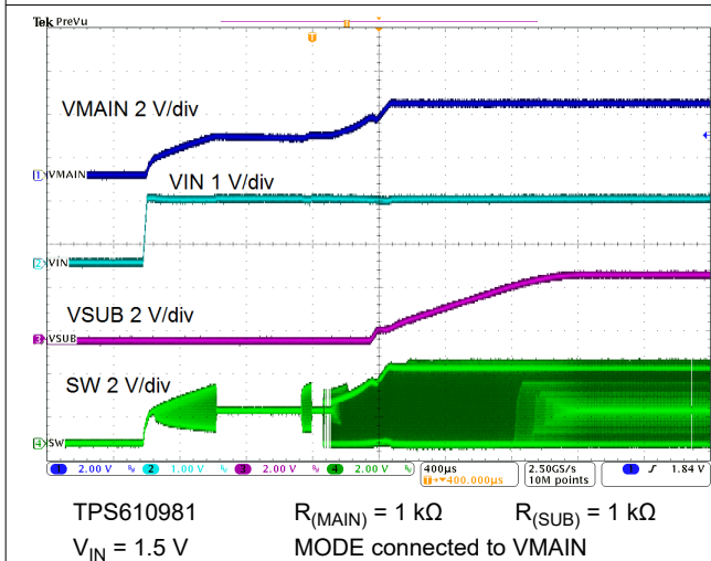
9-23. Startup
