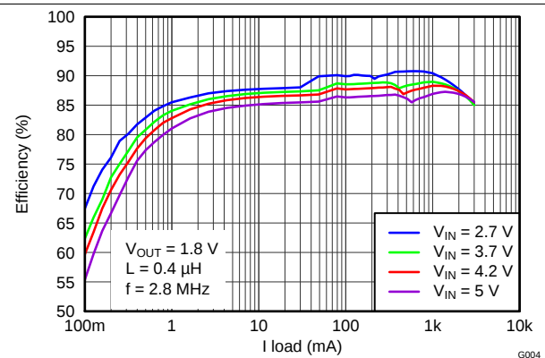
FIG 11. Efficiency vs Load Current
