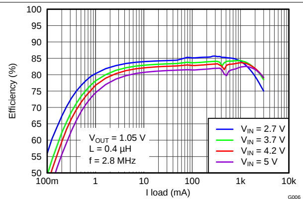
FIG 13. Efficiency vs Load Current
