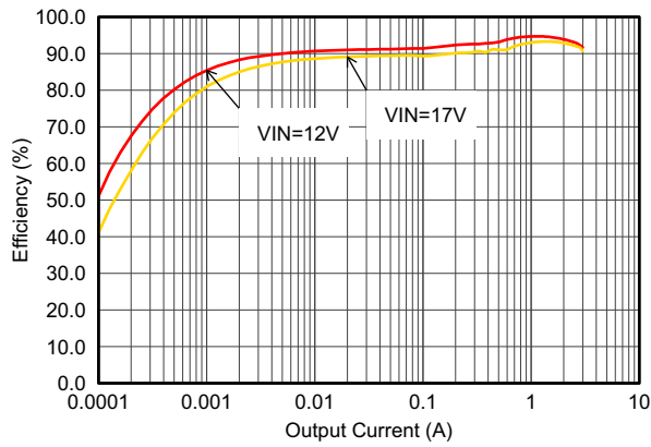
9-4. Efficiency with 1.25 MHz
