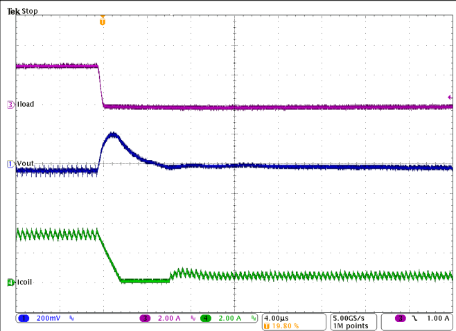
9-31. Load Transient Response
