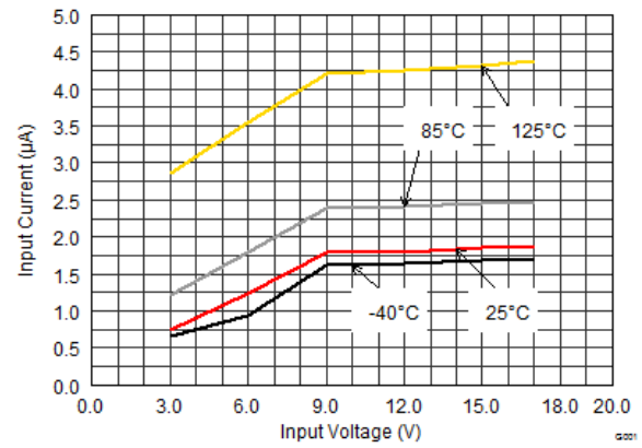
7-2. Shutdown Current
