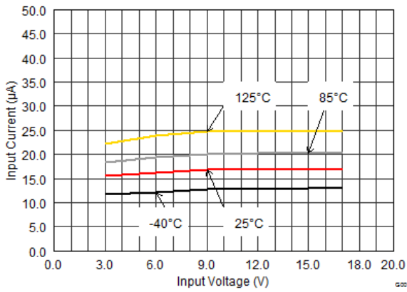
7-1. Quiescent Current
