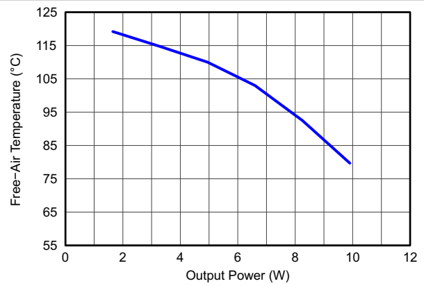
9-37. Typical Operation In Power Save Mode
