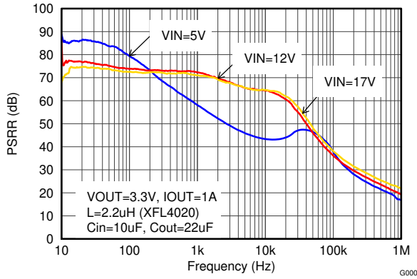
9-28. Power Supply Rejection Ratio
