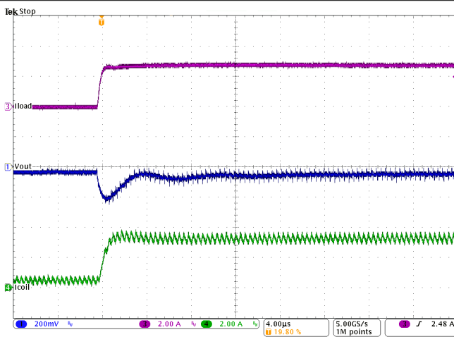
9-30. PWM-PSM-Transition
