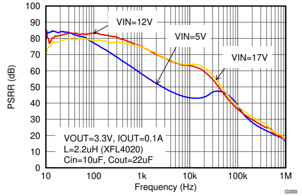
9-29. Power Supply Rejection Ratio
