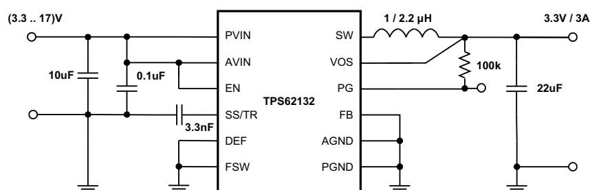
9-44. 3.3-V/3-A Power Supply
