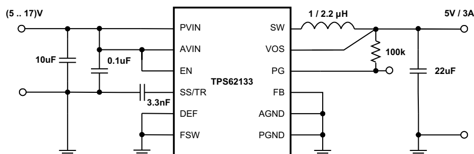
9-43. 5-V/3-A Power Supply
