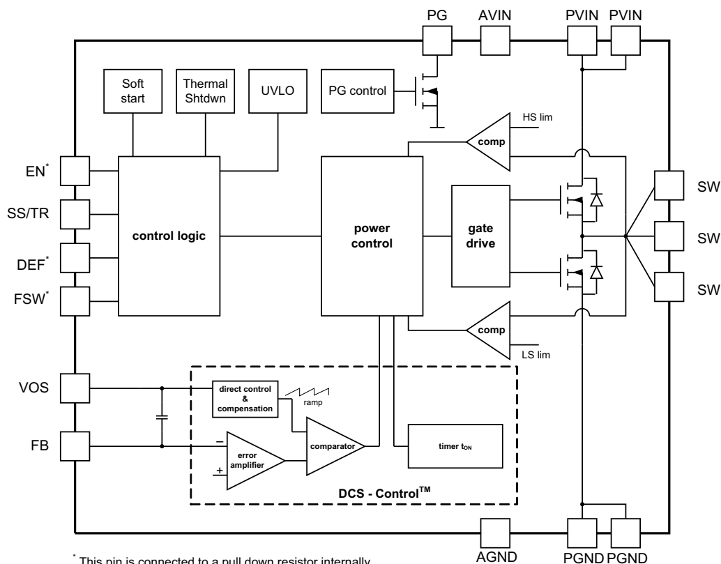
図 8-1. TPS62130 and TPS62130A (Adjustable Output Voltage)
