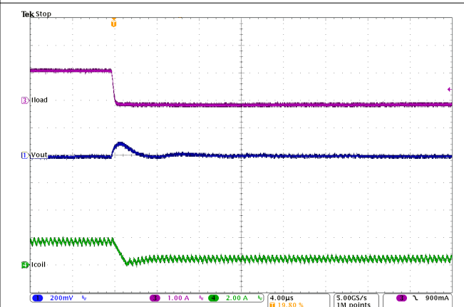
Figure 9-31. Load Transient Response
