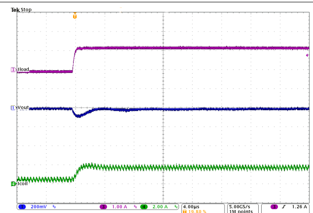
Figure 9-32. Line Transient Response of Figure 9-31, Rising Edge
