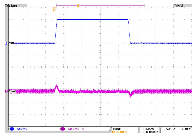
FIG 10-32. Line Transient Response
