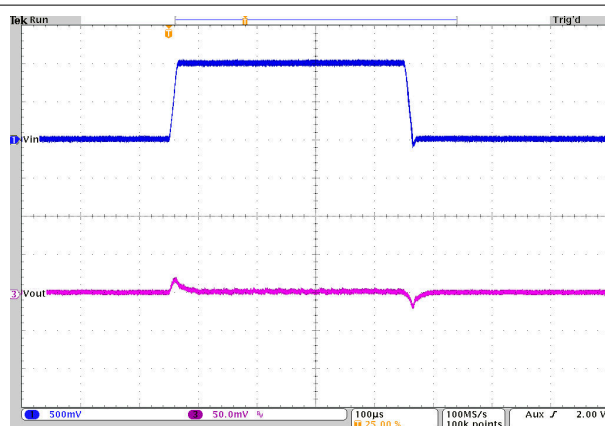
FIG 10-35. Line Transient Response
