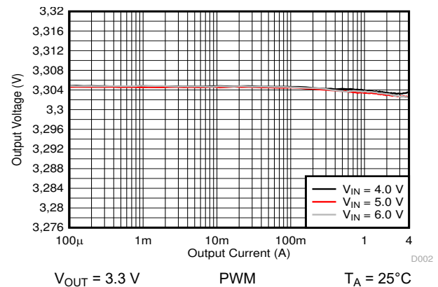
10-13. Output Voltage versus Output Current
