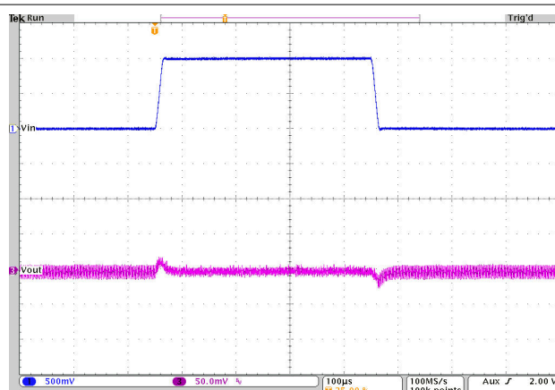
FIG 10-34. Line Transient Response
