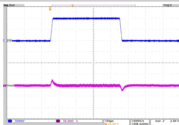
FIG 10-33. Line Transient Response
