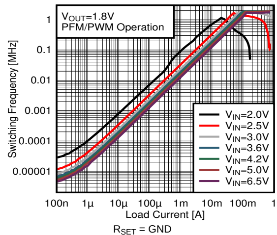
FIG 37. Switching Frequency versus Load Current V OUT = 1.8 V
