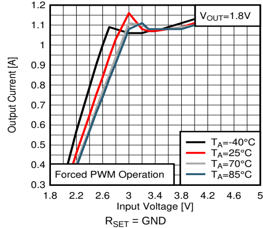
FIG 33. Maximum Output Current versus Input Voltage V OUT = 1.8 V
