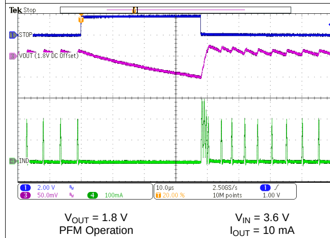
58. STOP Mode Operation
