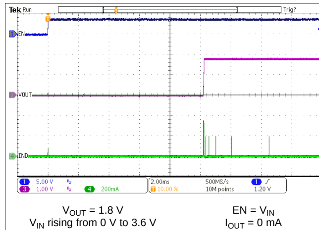
56. Start-up/Shutdown into No Load
