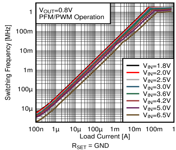
FIG 35. Switching Frequency versus Load Current V OUT = 0.8 V
