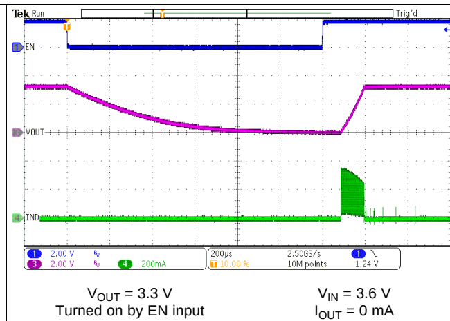
57. Start-up/Shutdown into No Load
