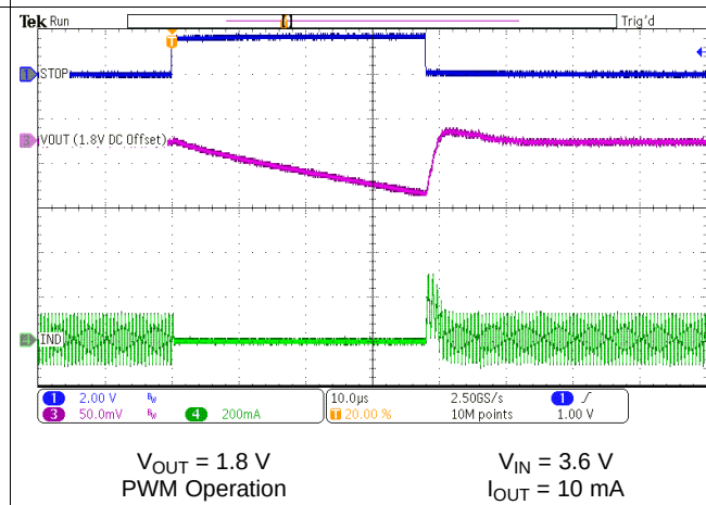
59. STOP Mode Operation
