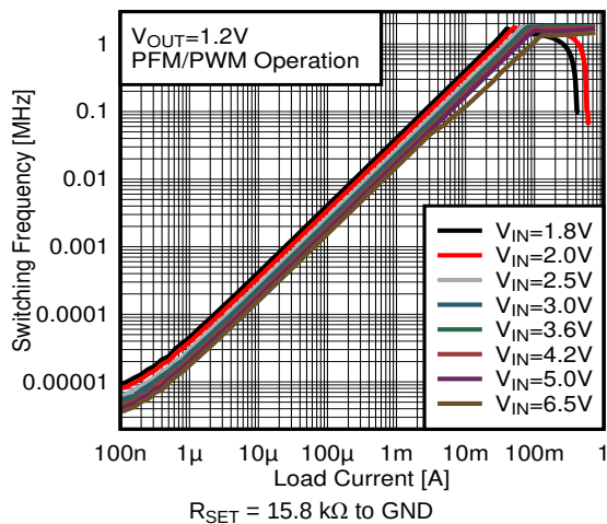
FIG 36. Switching Frequency versus Load Current V OUT = 1.2 V
