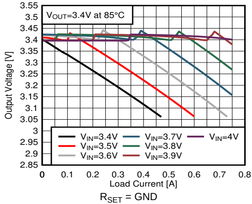
FIG 32. Output Voltage versus Load Current V OUT = 3.4 V
