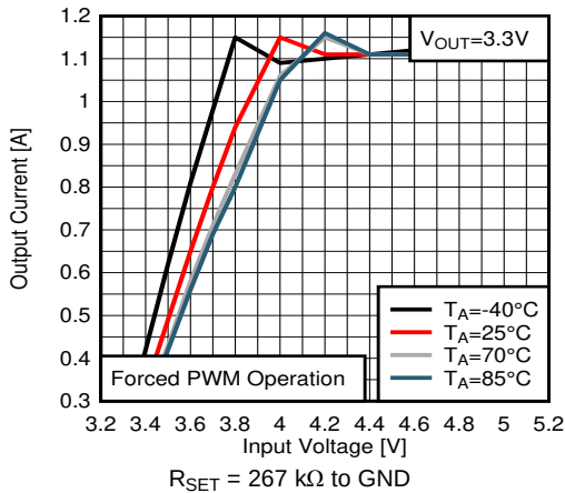
FIG 34. Maximum Output Current versus Input Voltage V OUT = 3.3 V
