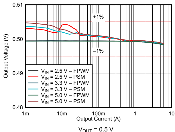
Figure 9-24. Load Regulation
