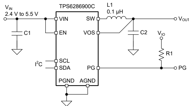
图 9-20. Typical Application
