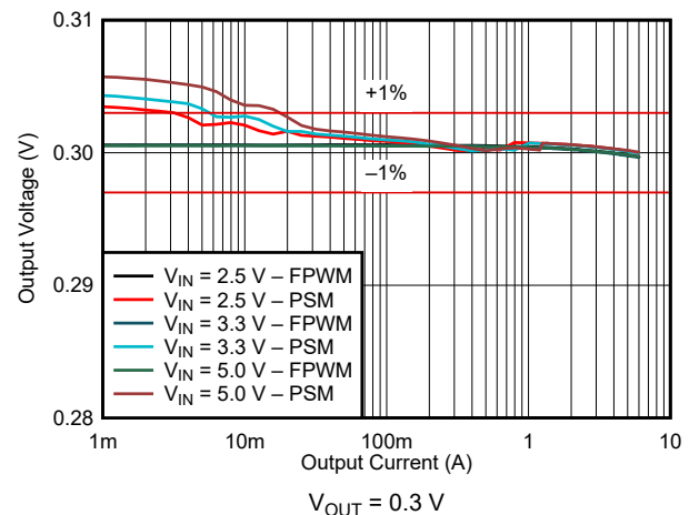
図 9-22. Load Regulation
