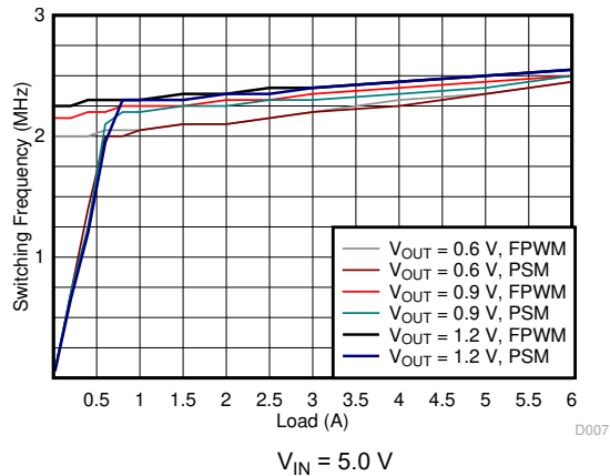
9-8. Switching Frequency
