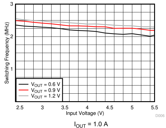
9-9. Switching Frequency
