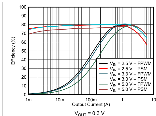
図 9-21. Efficiency
