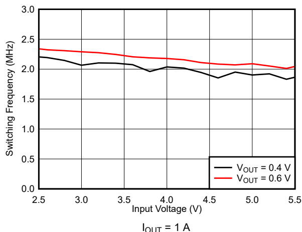
Figure 9-26. Switching Frequency
