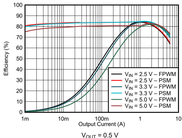
Figure 9-23. Efficiency
