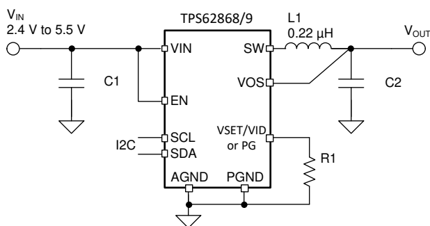
図 9-1. Typical Application
