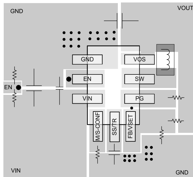
FIG 9-69. Layout
