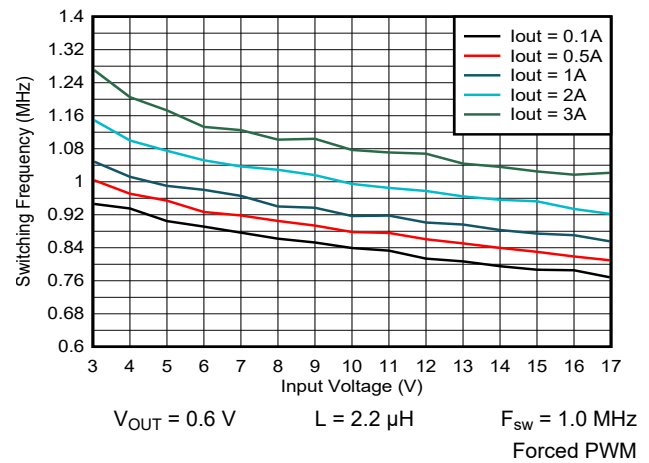
9-36. Switching Frequency vs Input Voltage
