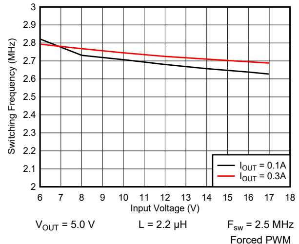
9-5. Switching Frequency vs Input Voltage
