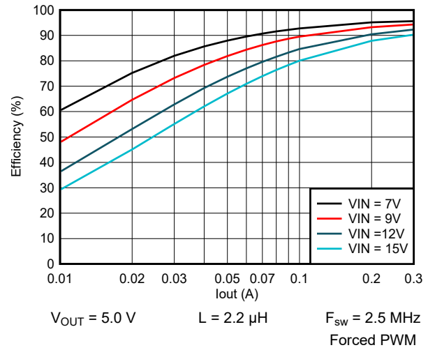
9-3. Efficiency vs Output Current
