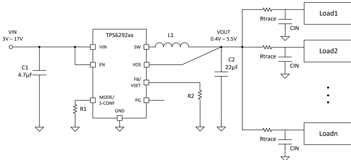
Figure 9-82. Multiple Loads Example
