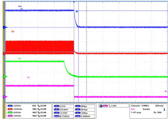
9-68. Shutdown Timing with Output Discharge Enabled
