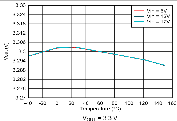
Figure 7-5. Output Voltage Accuracy – VSET Selected
