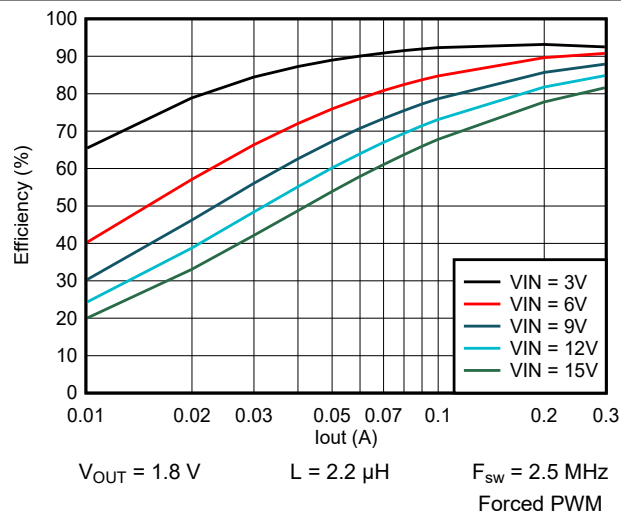
9-27. Efficiency vs Output Current
