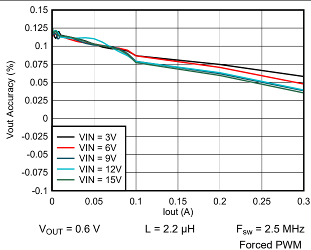
9-55. Output Voltage vs Output Current
