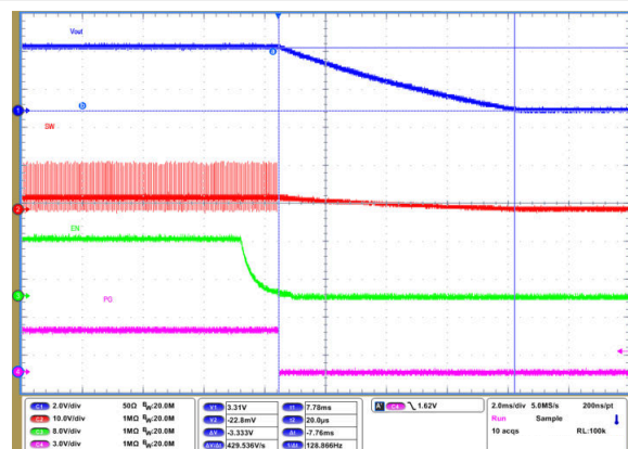
Figure 9-65. Shutdown Timing with Output Discharge Enabled
