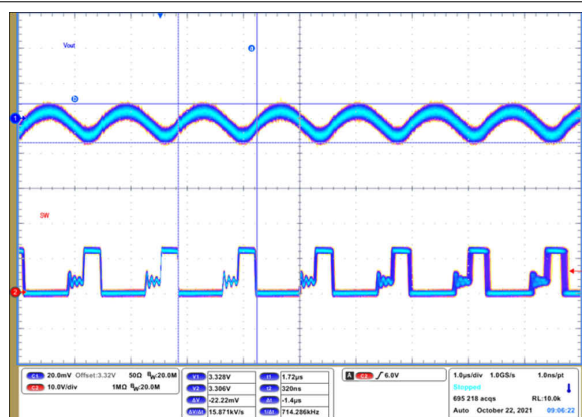
FIG 9-74. Output Voltage Ripple
