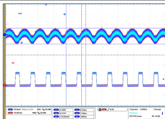
FIG 9-75. Output Voltage Ripple
