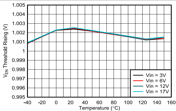
7-17. Precision Enable Threshold vs Temperature
