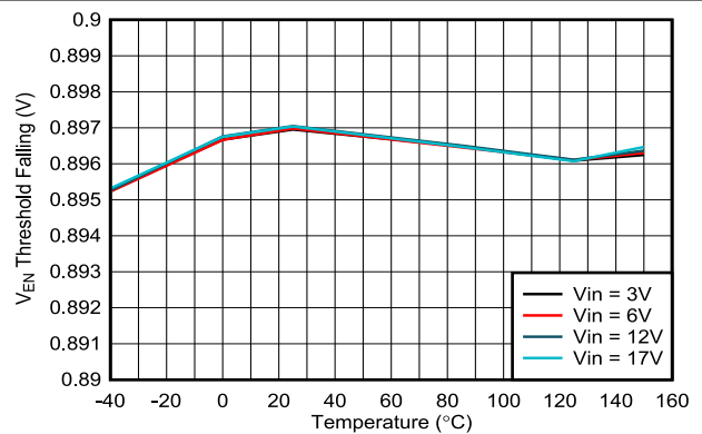
7-18. Precision Enable Threshold vs Temperature
