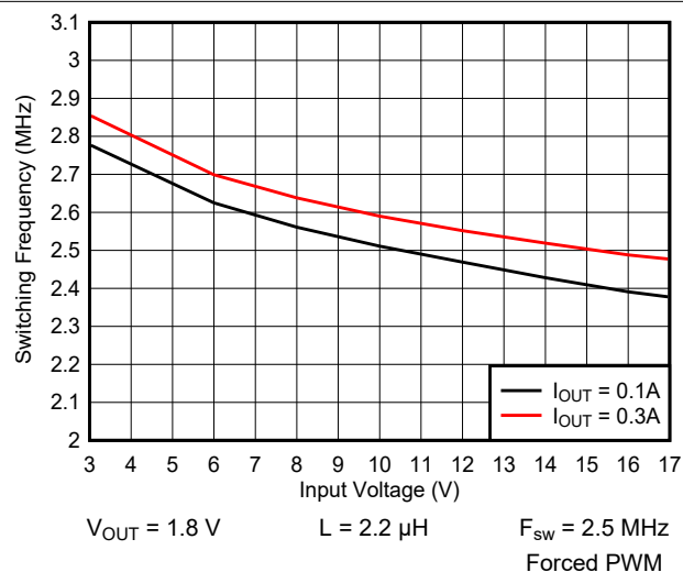
9-29. Switching Frequency vs Input Voltage
