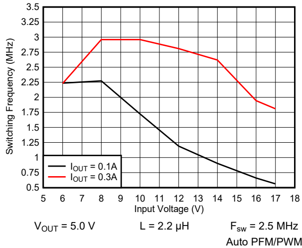
9-4. Switching Frequency vs Input Voltage
