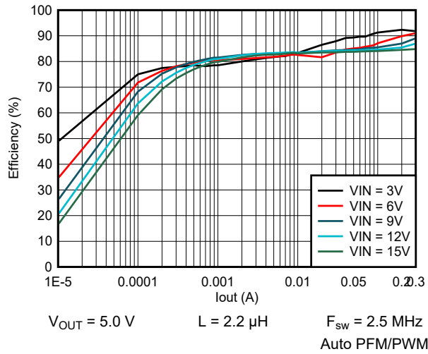
9-2. Efficiency vs Output Current
