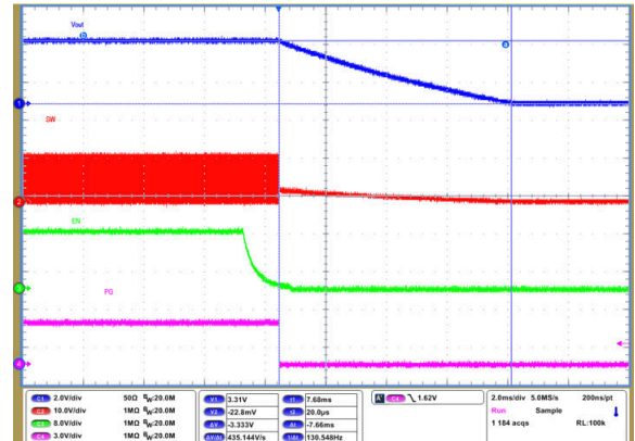
9-69. Shutdown Timing with Output Discharge Disabled
