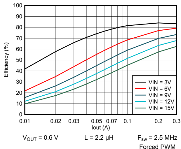
9-51. Efficiency vs Output Current
