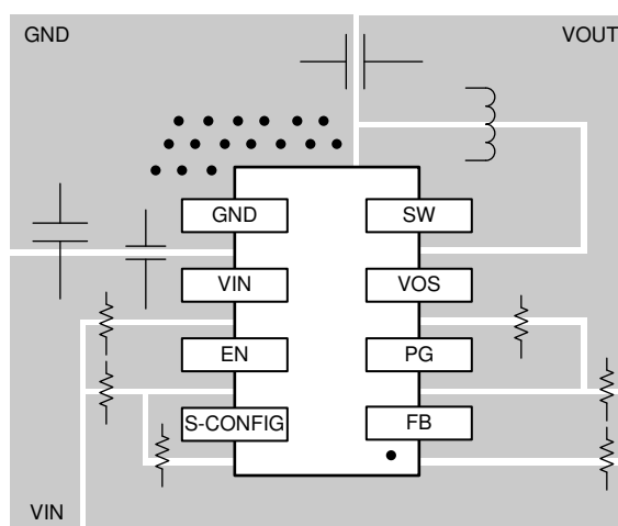
Figure 11-1. TPS629203-Q1 Layout
