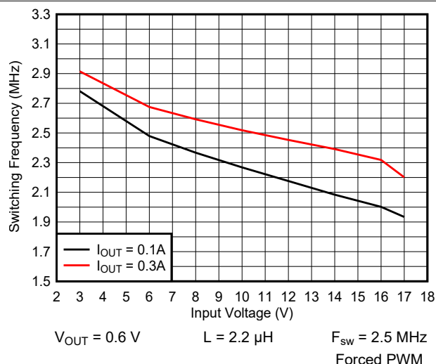
9-53. Switching Frequency vs Input Voltage
