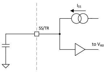
FIG 9-2. Soft-Start Operation Simplified Schematic
