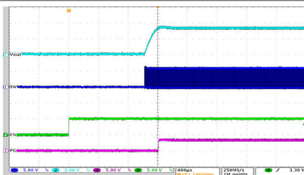
图 9-65. Start-Up Timing
