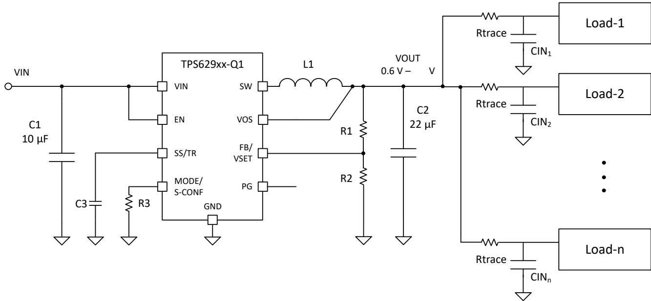
9-82. Multiple Loads
