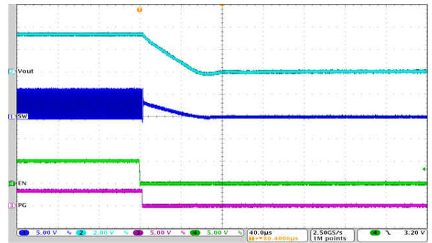
图 9-71. Shutdown Timing with Output Discharge Disabled
