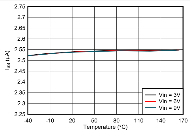
Figure 7-18. Soft Start Current vs Temperature
