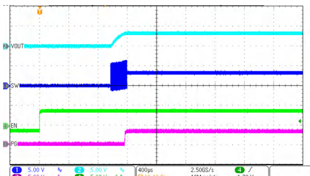
图 9-65. Start-Up Timing
