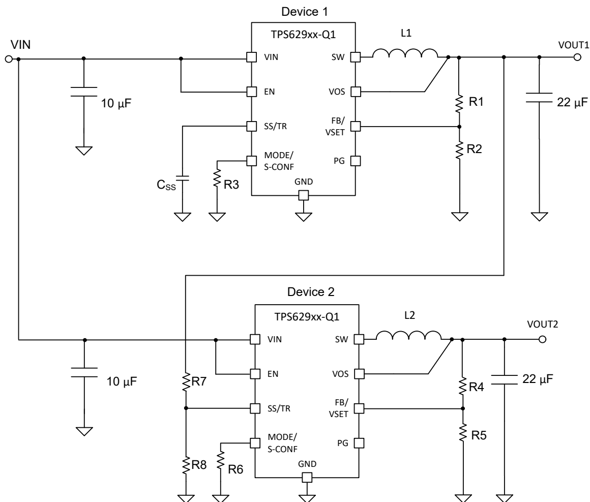
FIG 9-83. Tracking Example
