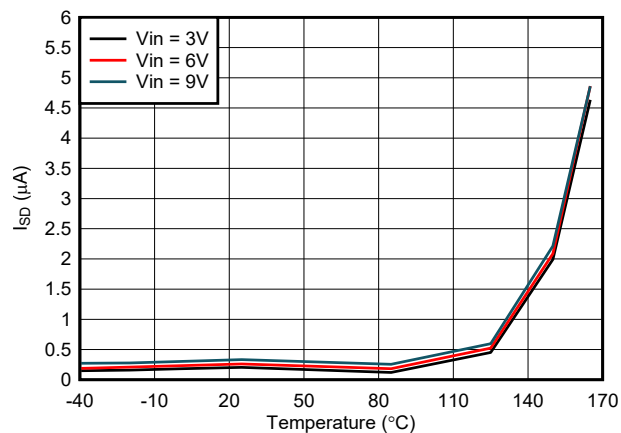
FIG 7-2. Shutdown Current vs Temperature
