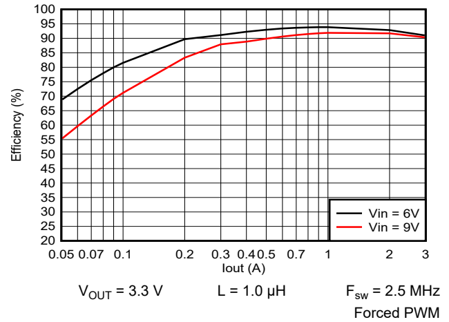
9-53. Efficiency vs Output Current
