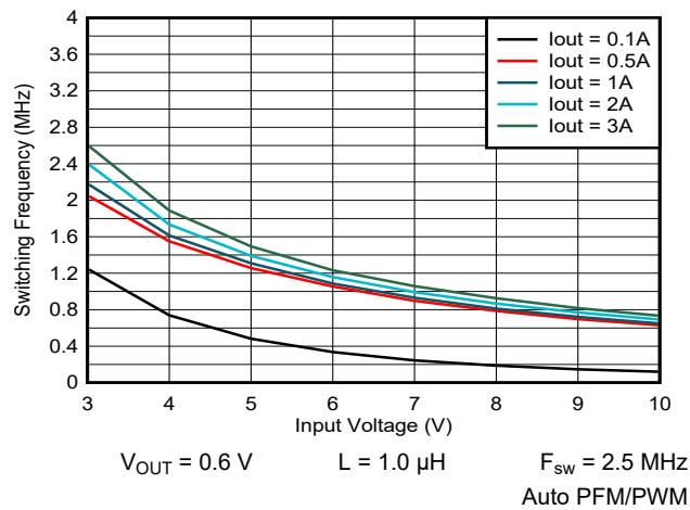
9-29. Switching Frequency vs Input Voltage
