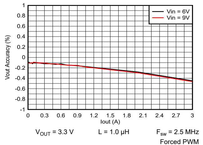
9-57. Output Voltage vs Output Current
