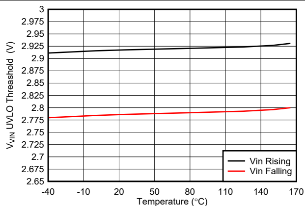
7-20. V_{VIN} UVLO Thresholds vs Temperature
