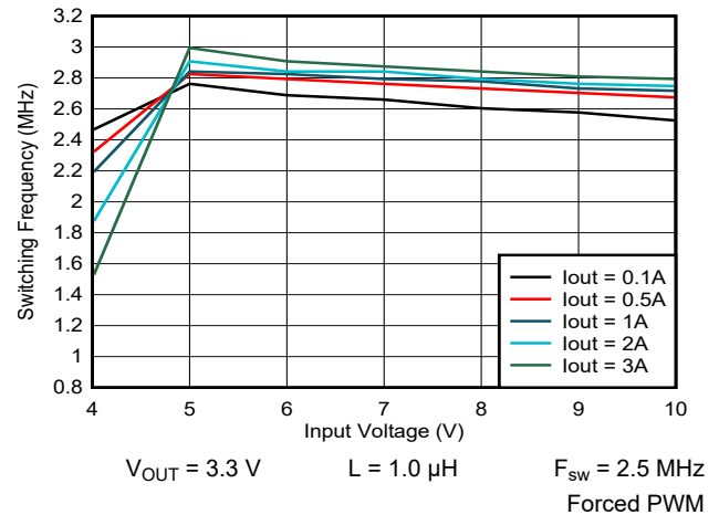
9-55. Switching Frequency vs Input Voltage
