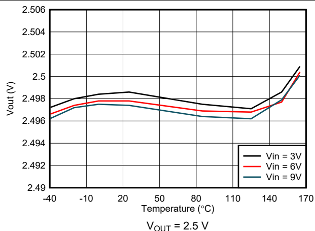
FIG 7-6. Output Voltage Accuracy - VSET Selected
