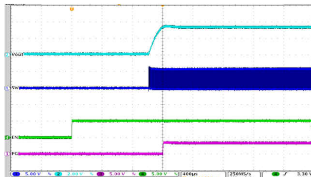
Figure 9-65. Start-Up Timing
