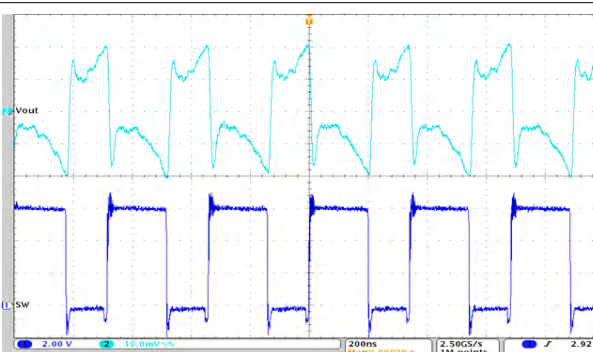
9-77. Output Voltage Ripple
