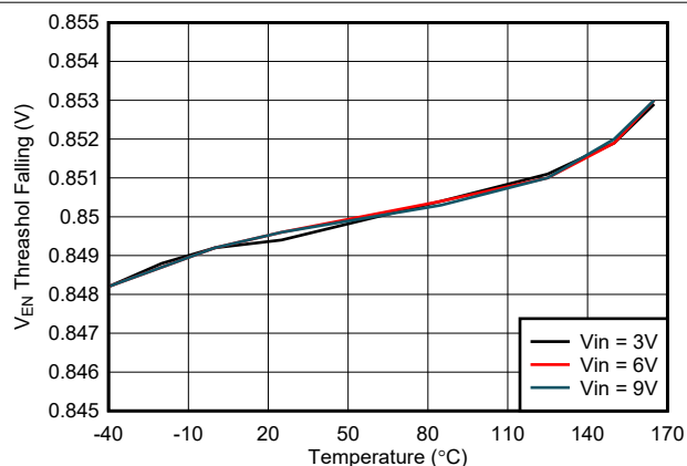
7-22. Percise EN Threshold vs Temperature
