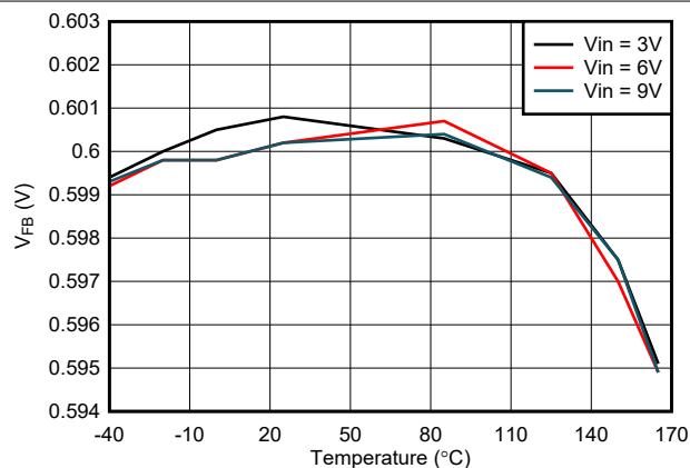
FIG 7-3. Feedback Voltage Accuracy - External Feedback Selected
