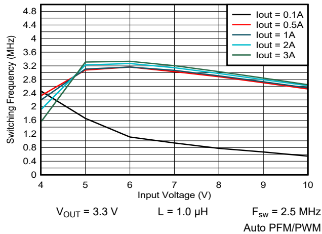
9-54. Switching Frequency vs Input Voltage
