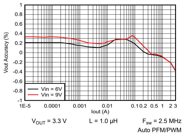
9-56. Output Voltage vs Output Current
