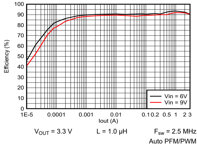
9-52. Efficiency vs Output Current
