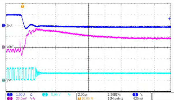
图 9-72. Load Transient Response
