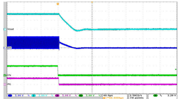
图 9-71. Shutdown Timing with Output Discharge Disabled
