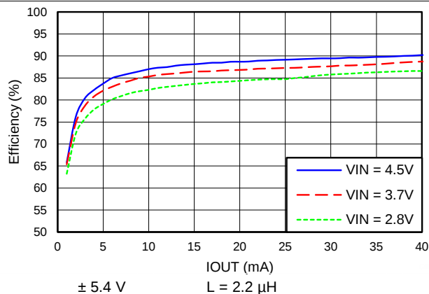
Figure 23. Combined Efficiency — 40mA Mode
