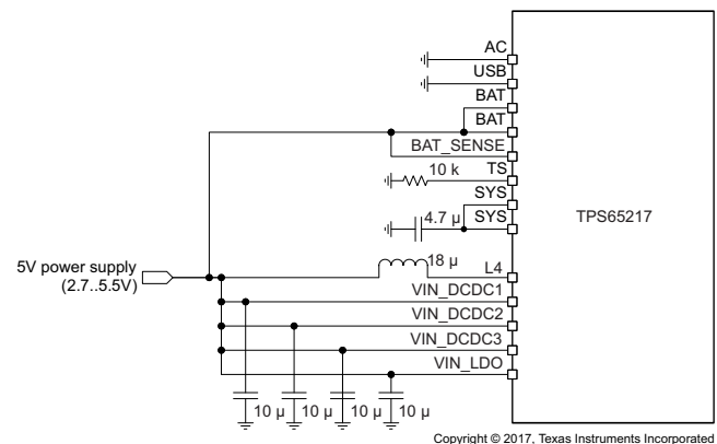
Figure 62. Power Connection for 5-V Only Operation Directly Wired to BAT Instead of a Battery
