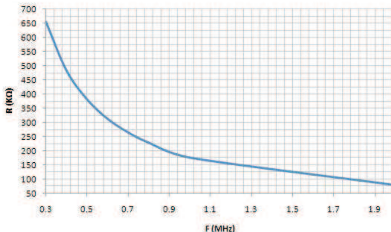
Figure 15. ROOSC vs Switching Frequency
