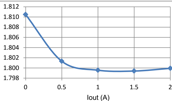
Figure 6-10. Load Regulation, 25°C, 1% 100-PPM Resistor
