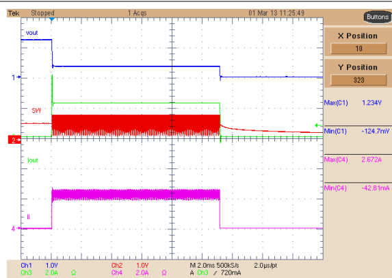
8-18. Buck 1 Current Limit Operation, Hiccup
