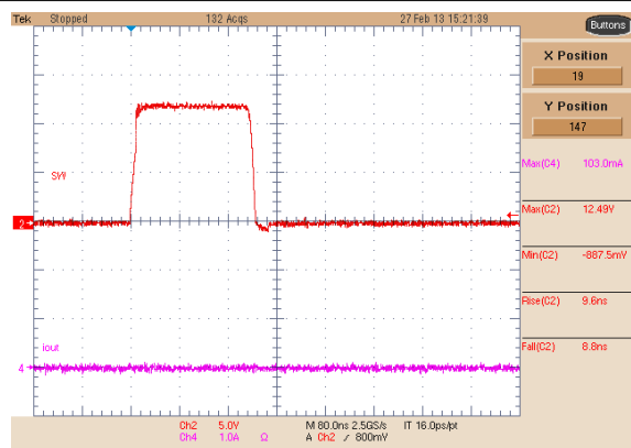
Figure 8-7. Buck 1 Switching Node, No Load
