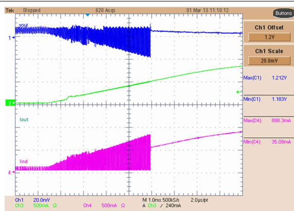
8-20. Buck 1 Low-Power Operation
