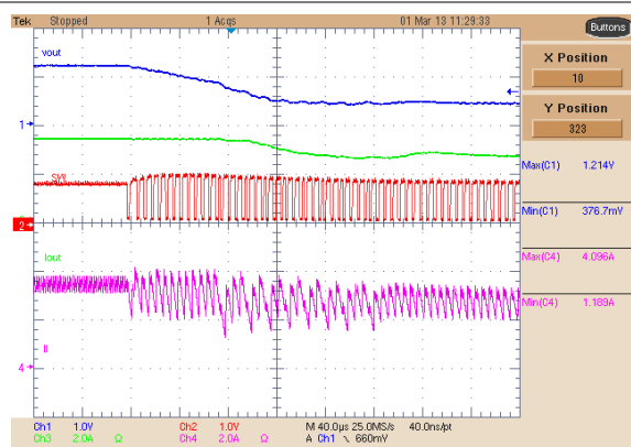
8-17. Buck 1 Current Limit Operation With Slow Rising Output Current, Trip at 4 A
