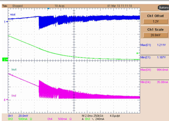
8-19. Buck 1 Low-Power Output, No Load
