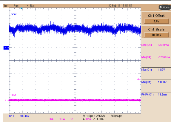
8-30. Buck 2 Ripple, No Load
