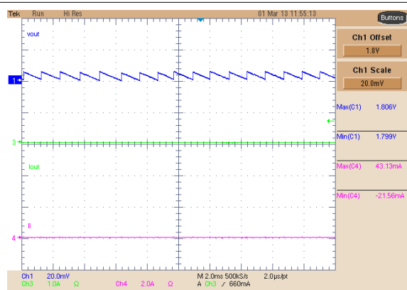
8-33. Buck 2 Low-Power Output, No Load
