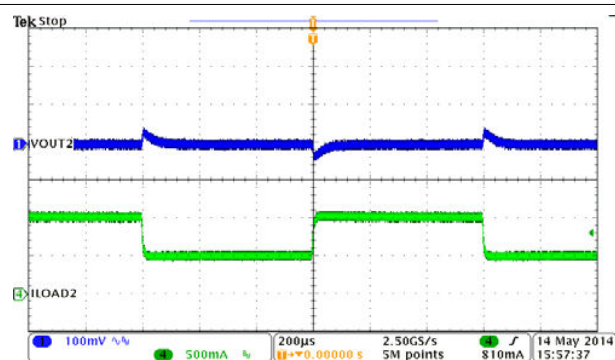
图 9-10. BUCK2, Load Transient, 0.5 to 1 A SR = 0.25 A/µs
