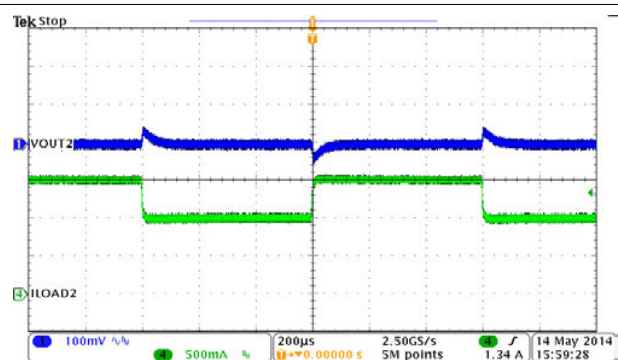
图 9-11. BUCK2, Load Transient, 1 to 1.5 A SR = 0.25 A/µs
