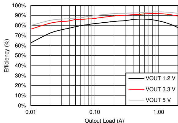
图 7-2. BUCK2 Efficiency
