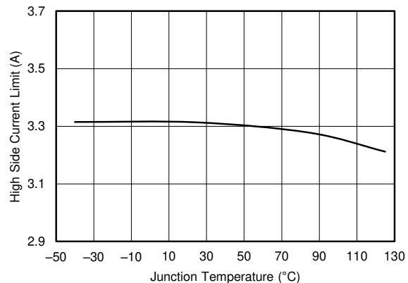
FIG 7-20. Buck3 High-Side Current Limit vs Temperature
