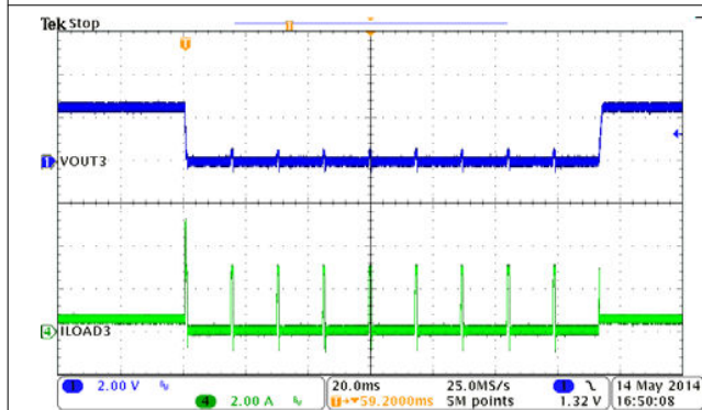
図 9-16. BUCK3, Hiccup and Recovery
