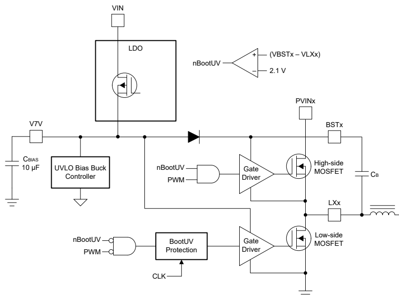
8-9. V7V Linear Dropout Regulator and Bootstrap Voltage Diagram
