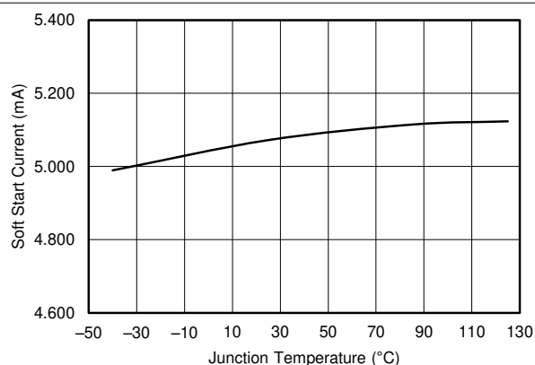
FIG 7-17. SS Pin Charge Current vs Temperature
