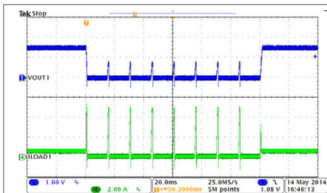
図 9-14. BUCK1, Hiccup and Recovery
