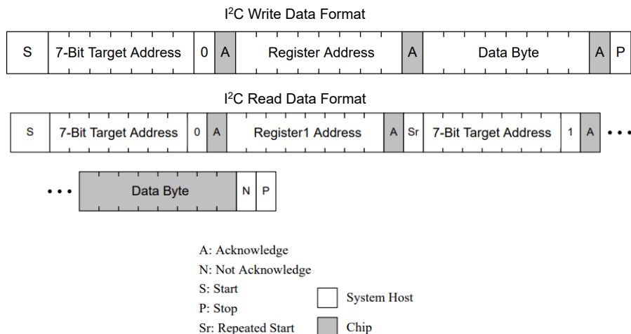
图 8-13. I²C Write and Read Data Format
