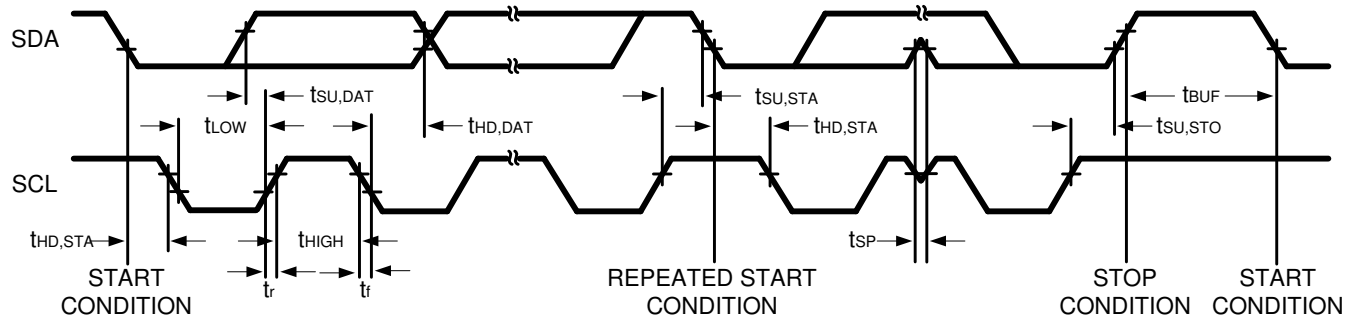
图 8-12. I²C Interface Timing Diagram
