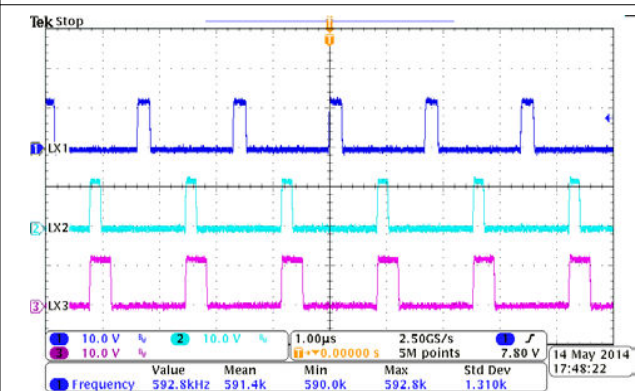
図 9-17. 180° Out-of-Phase
