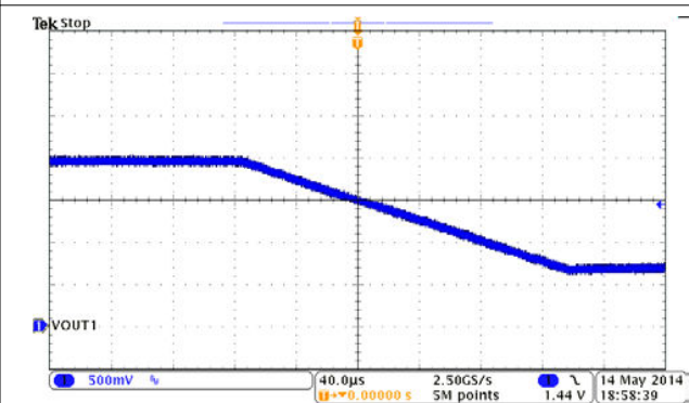
図 9-19. VID1 from 7F to 00, SR = 10 mV/cycle
