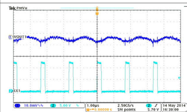
図 9-5. BUCK1, Output Voltage Ripple, Iout = 3 A
