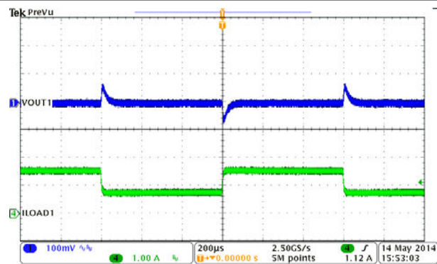
图 9-8. BUCK1, Load Transient, 0.75 to 1.5 A SR = 0.25 A/µs
