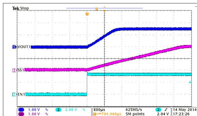
図 9-2. BUCK1, Soft-Start, Iout = 3 A
