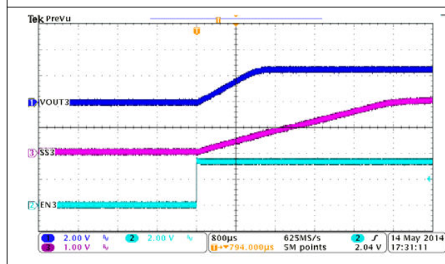
図 9-4. BUCK3, Soft-Start, Iout = 2 A
