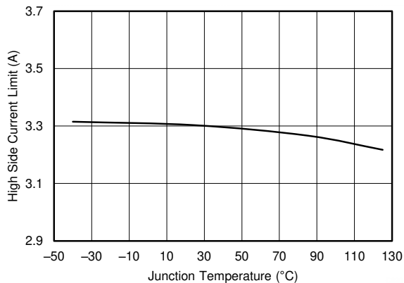
FIG 7-19. Buck2 High-Side Current Limit vs Temperature
