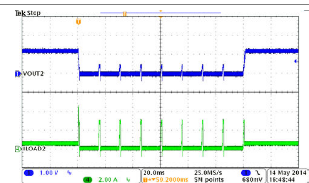
図 9-15. BUCK2, Hiccup and Recovery
