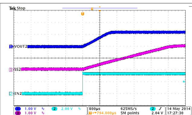
図 9-3. BUCK2, Soft-Start, Iout = 2 A
