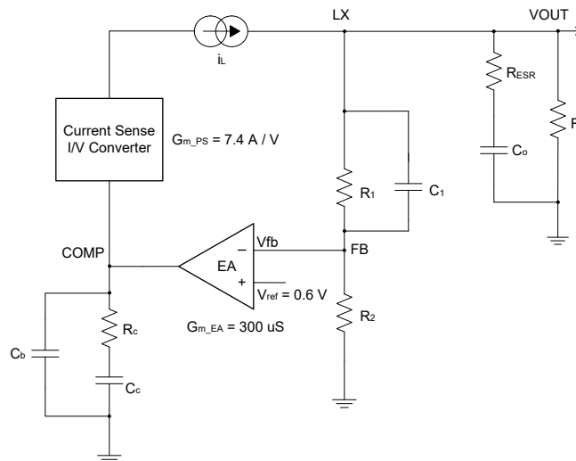
FIG 9-1. DC/DC Loop Compensation
