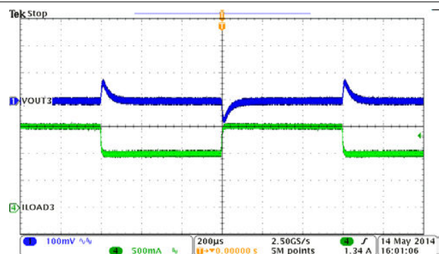
图 9-13. BUCK3, Load Transient, 1 to 1.5 A SR = 0.25 A/µs
