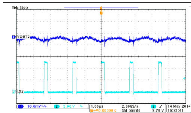
図 9-6. BUCK2, Output Voltage Ripple, Iout = 3 A
