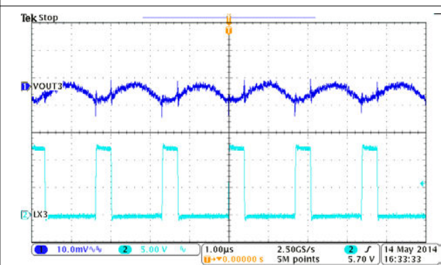
図 9-7. BUCK3, Output Voltage Ripple, Iout = 2 A
