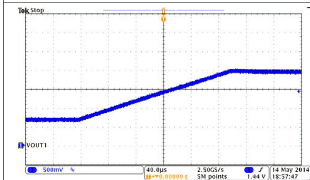
図 9-18. VID1 from 00 to 7F, SR = 10 mV/cycle
