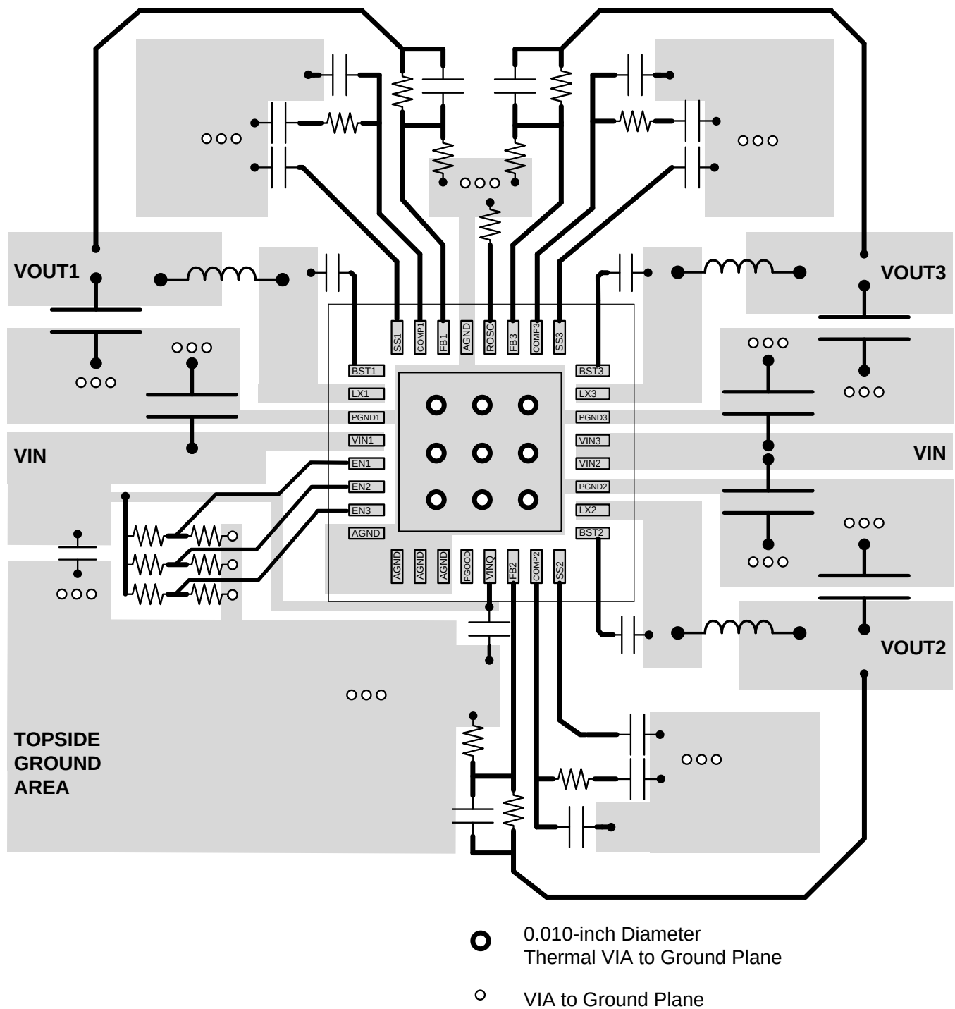
Figure 51. PCB Layout
