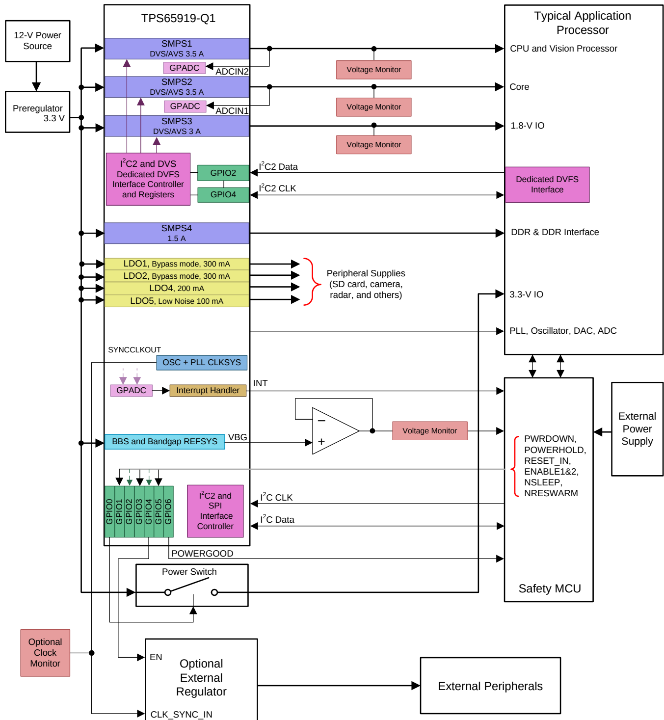
FIG 6-1. Application Diagram in a Typical ADAS System
