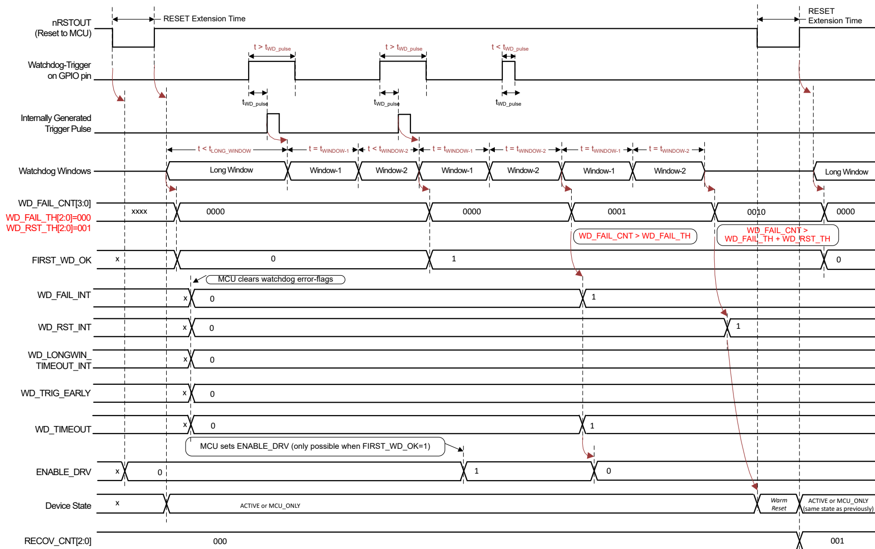
図 8-19. Watchdog in Trigger Mode – Bad Events (Too Short or no Trigger in Window-2) After Start-up
