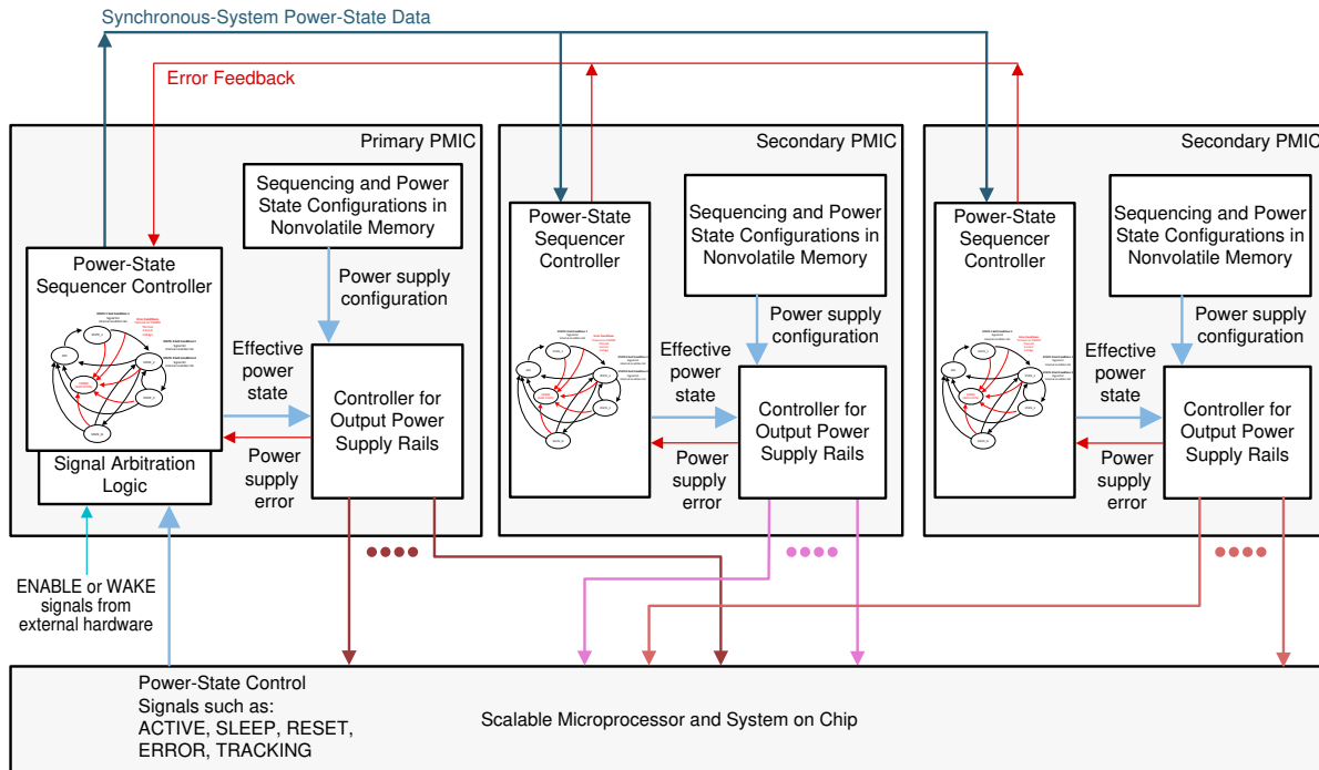
8-43. Multi-PMIC Power State Synchronization Block Diagram
