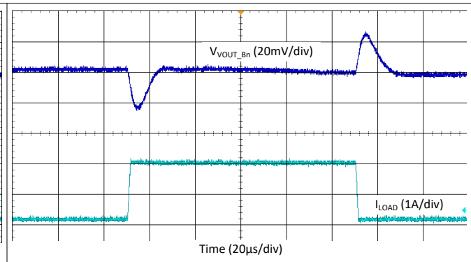
図 9-53. Buck Load Step Transient - Buck4, 4.4 MHz, Forced-PWM Mode
