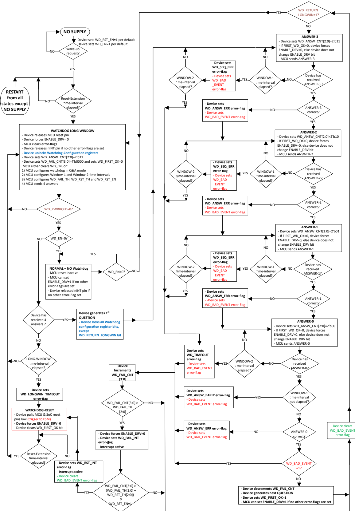
図 8-24. Flow Chart for WatchDog in Q&A Mode
