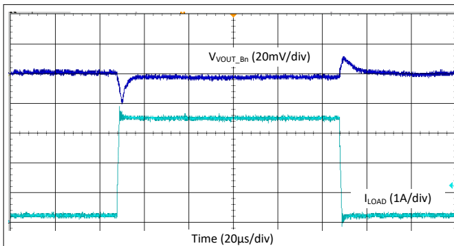
図 9-46. Buck Load Step Transient - 2-Phase, 2.2 MHz, Auto Mode
