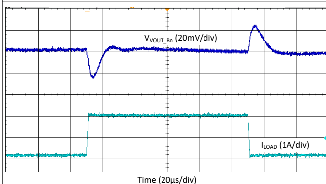
図 9-48. Buck Load Step Transient - 2-Phase, 2.2 MHz, Forced-PWM Mode
