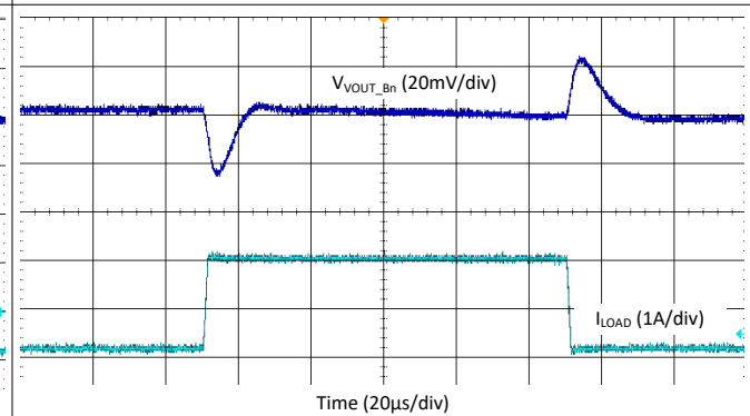
図 9-49. Buck Load Step Transient - 2-Phase, 4.4 MHz, Forced-PWM Mode
