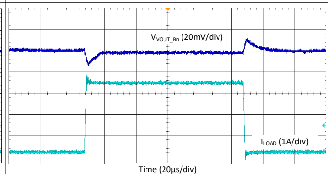
図 9-47. Buck Load Step Transient - 2-Phase, 4.4 MHz, Auto Mode
