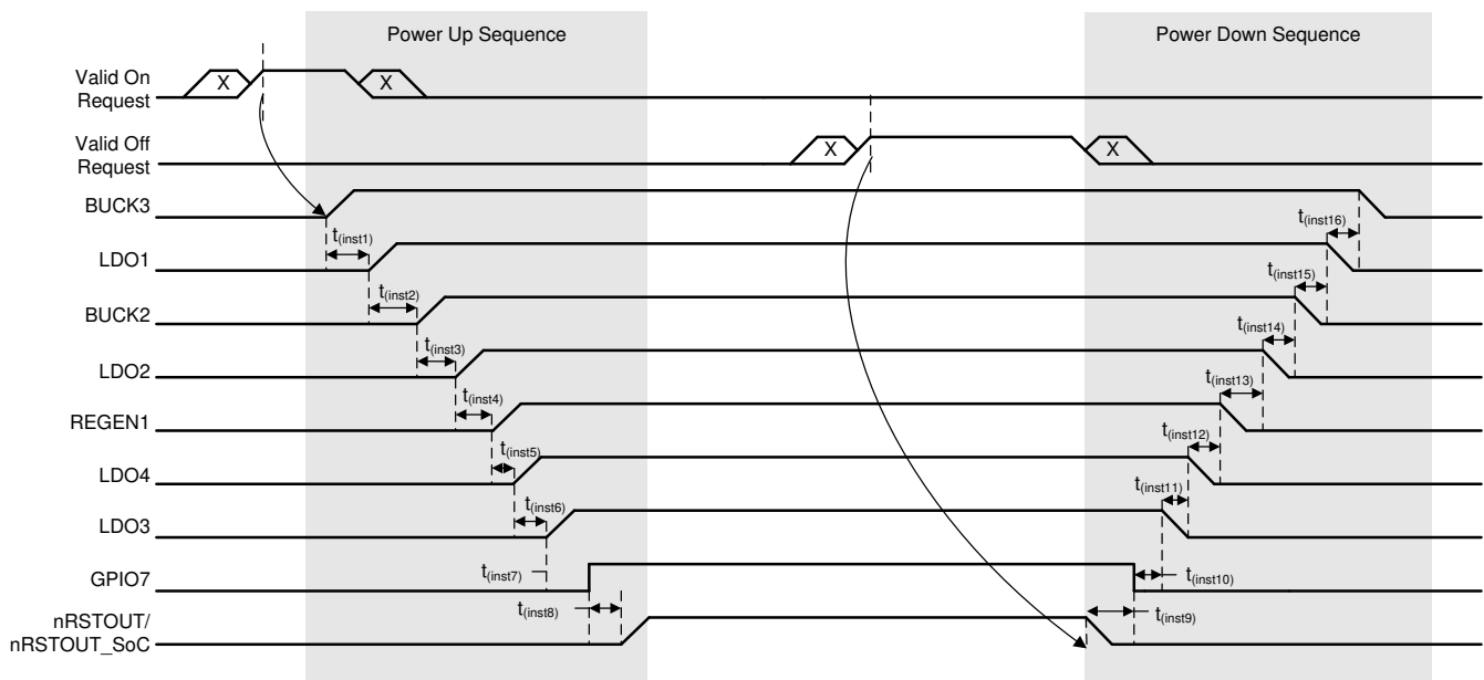
図 8-42. Power Sequence Example
