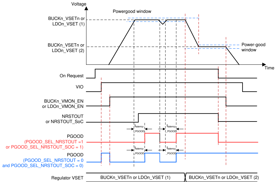
8-11. PGOOD Waveforms
