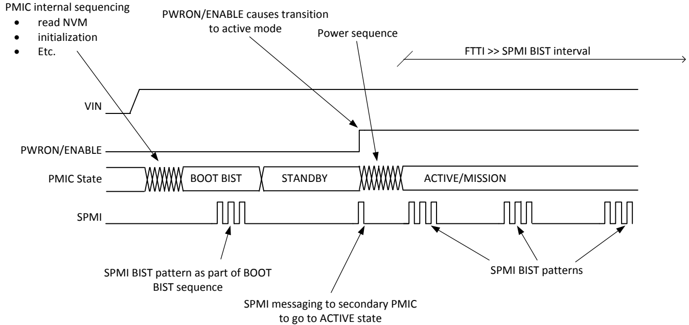
8-50. SPMI-BIST Operation
