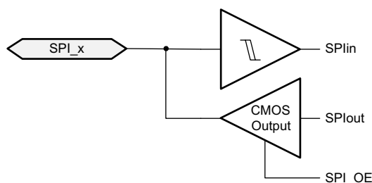
Figure 9-50. IOBUF_GPIOHSSI
