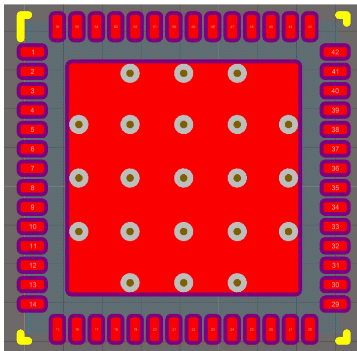
FIG 12-1. Top View Standard TPS65981 Footprint
