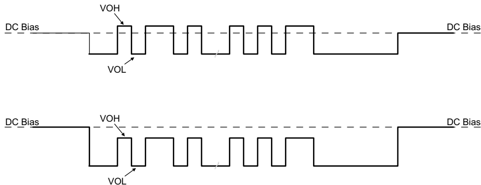
FIG 9-6. TX Driver Transmission with DC Bias
