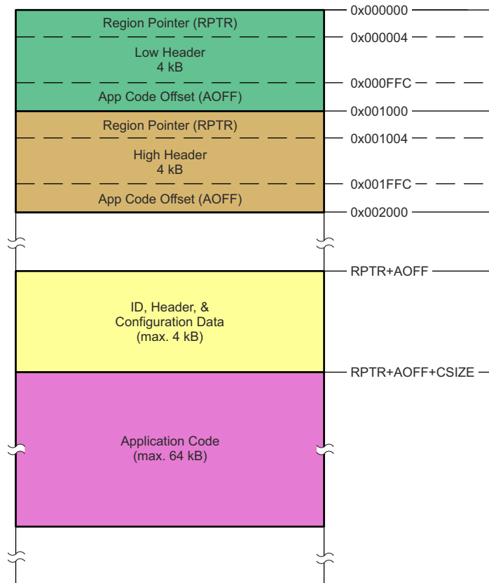
FIG 9-55. Flash Memory Organization
