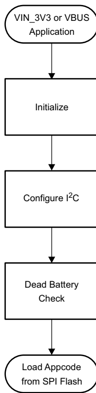
FIG 9-52. Flow Diagram for Boot Code Sequence
