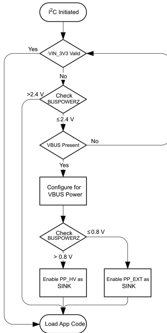
FIG 9-54. Dead-Battery Condition Flow Diagram
