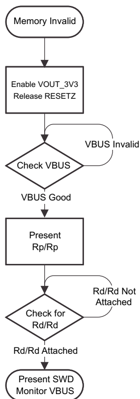
FIG 9-57. Memory Invalid Flow
