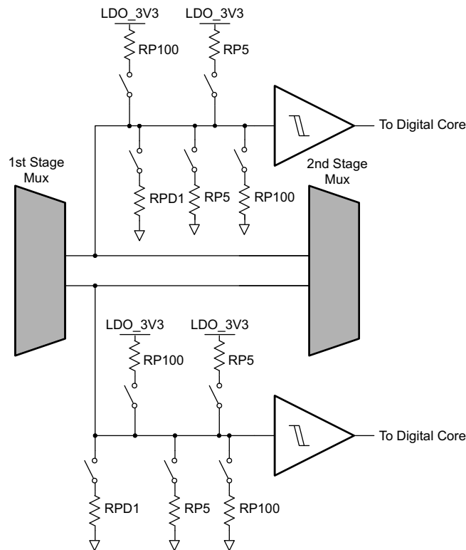
FIG 9-36. Port Detect and Pull-up and Pull-down
