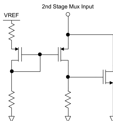
FIG 9-37. Port Multiplexer Clamp
