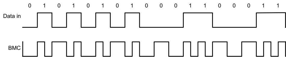
FIG 9-4. Biphasic Mark Coding Example
