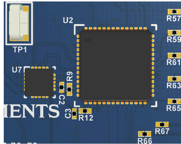
✎ 12-5. Example Layout (Top View in 3-D)
