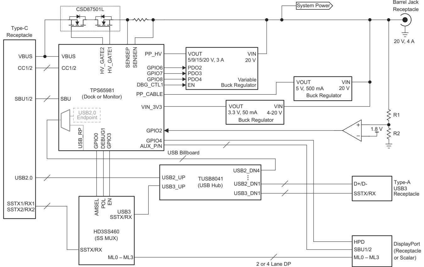
图 10-3. Type-C and PD Dock or Monitor Application
