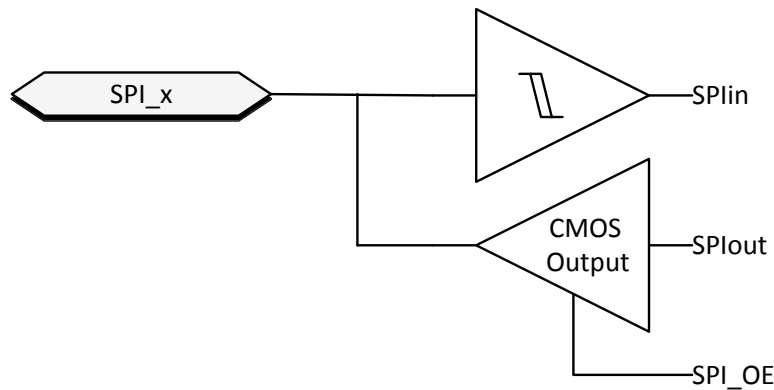
図 8-21. SPI buffer
