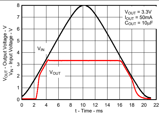
Figure 5-25. Power-Up, Power-Down (New Chip)
