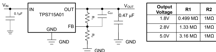
図 7-2. TPS715A01 Adjustable LDO Regulator Programming
