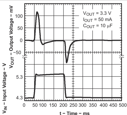
7-6. Fast Power-Up (Legacy Chip)
