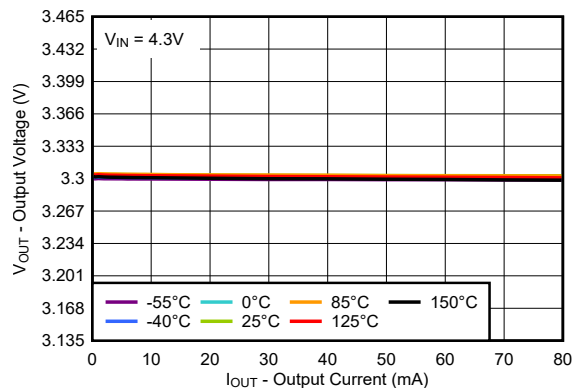
図 5-2. TPS715A33 Output Voltage vs Output Current (New Chip)
