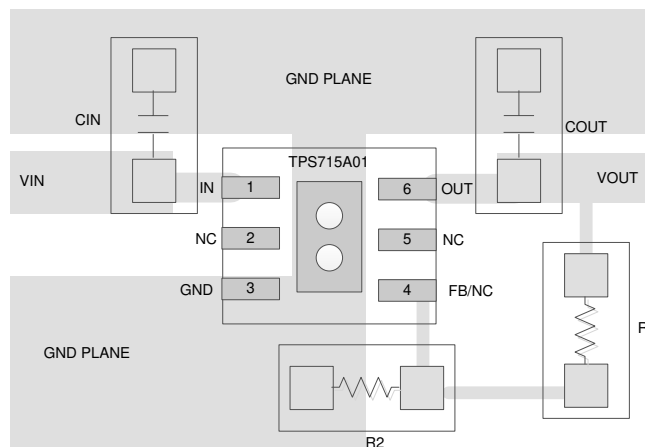
図 7-14. Example Layout for the TPS715A01DRV
