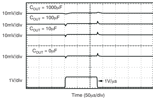
FIG 5-29. V_{BIAS} Line Transient (1.5A) (legacy chip)
