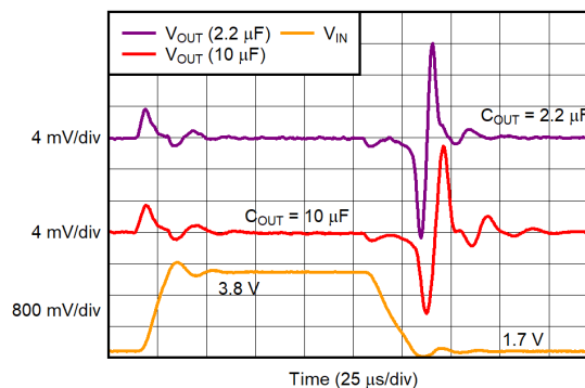
图 5-32. V_{IN} Line Transient (new chip)
