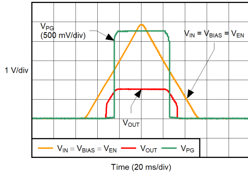
図 5-37. Power-Up, Power-Down (new chip)
