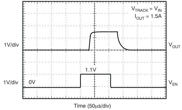
図 5-38. Turn-On Response (legacy chip)
