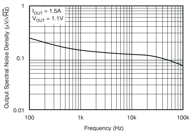
图 5-20. Noise Spectral Density (legacy chip)
