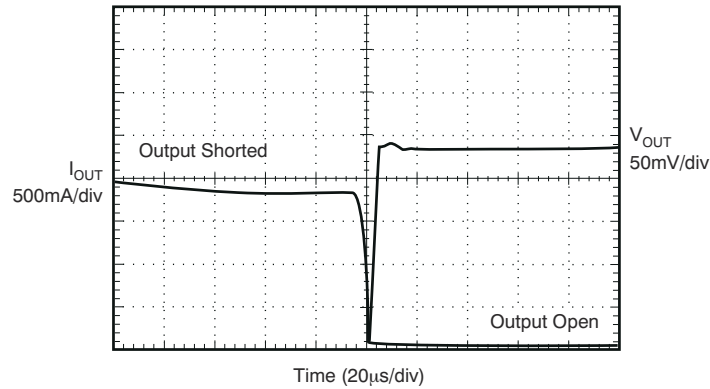
図 5-39. Output Short Circuit Recovery
