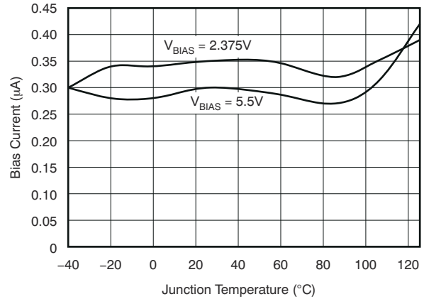
FIG 5-26. I_{BIAS} Shutdown vs Temperature (legacy chip)
