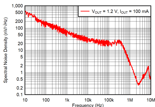
图 5-21. Noise Spectral Density (new chip)
