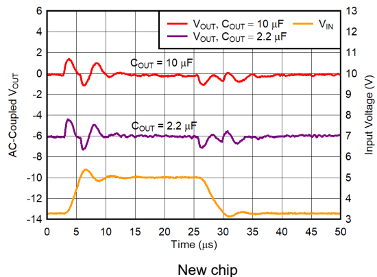
FIG 5-30. V_{BIAS} Line Transient (new chip)
