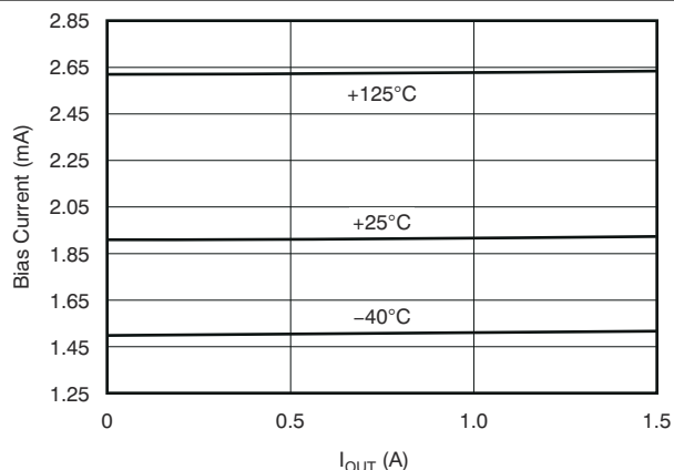
图 5-22. I_{BIAS} vs I_{OUT} and Temperature (legacy chip)
