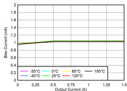
图 5-23. BIAS Pin Current vs Output Current and Temperature ( T_J ) (new chip)
