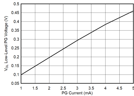
FIG 5-28. Low-Level PG Voltage vs Current (new chip)
