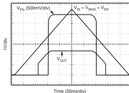
图 5-36. Power-Up/Power-Down (legacy chip)
