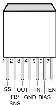
図 4-2. KTW PACKAGE DDPACK-7 SURFACE-MOUNT (Legacy only)
