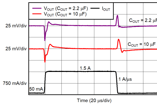
図 7-7. Output Load Transient Response (new chip)
