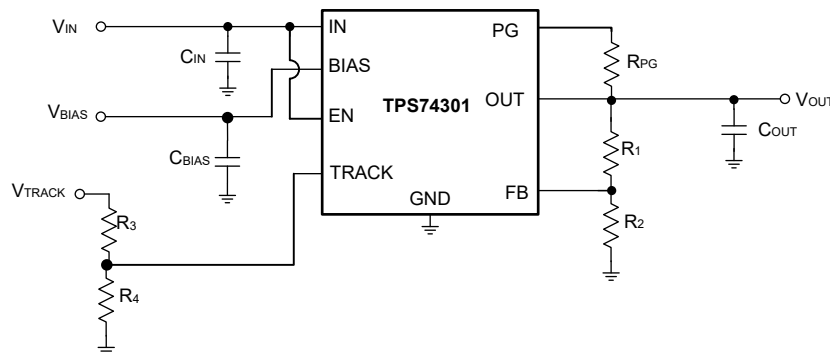
図 7-4. Typical Application Circuit for the TPS74301
