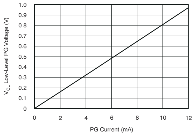
FIG 5-27. Low-Level PG Voltage vs PG Current (legacy chip)
