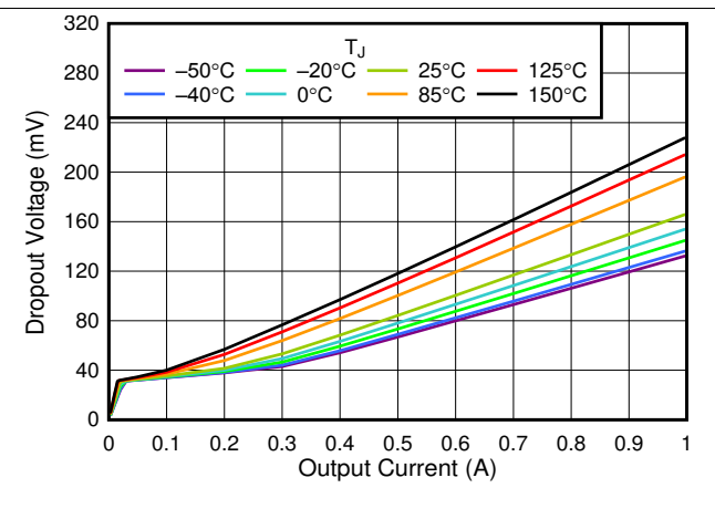
Fig. 4. 3.3-V Dropout Voltage vs I_{OUT}
