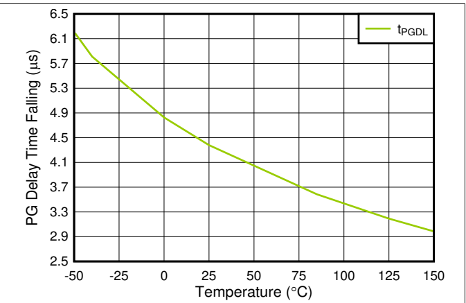
20. t_{PGDL} vs Temperature
