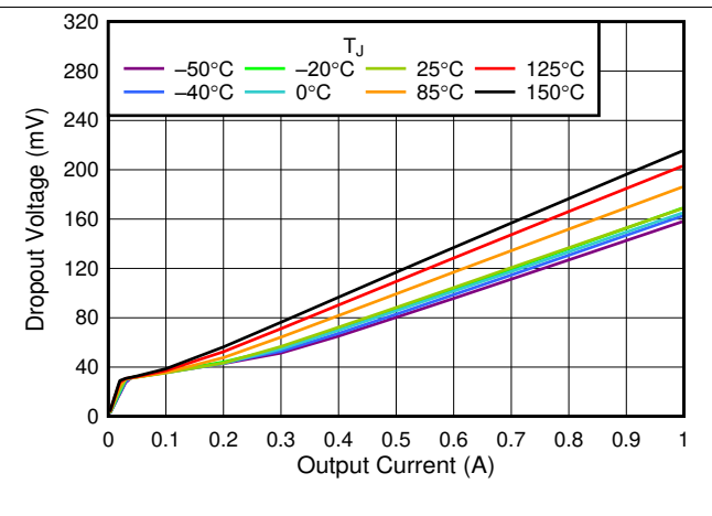
Fig. 6. 5.5-V Dropout Voltage vs I_{OUT}
