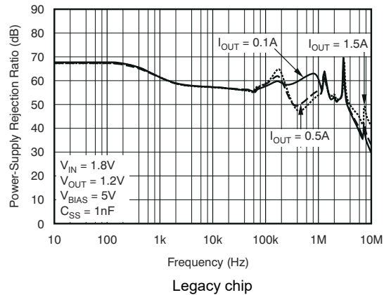
Figure 5-15. V_{BIAS} PSRR vs Frequency
