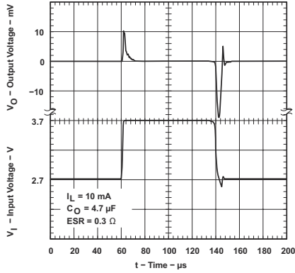
図 5-37. TPS76915 Line Transient Response (Legacy Chip)
