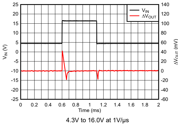
図 5-41. TPS76933 Line Transient Response (New Chip)
