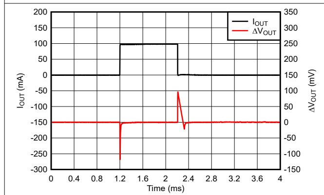
1mA to 100mA at 1A/μs
