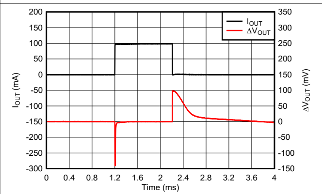
1μA to 100mA at 1A/μs
