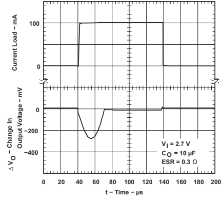
図 5-38. TPS76915 Load Transient Response (Legacy Chip)
