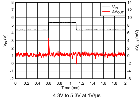
図 5-40. TPS76933 Line Transient Response (New Chip)
