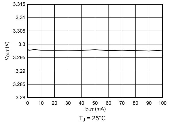
図 5-4. TPS76933 Output Voltage vs Output Current (New Chip)
