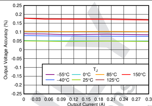
6-2. Output Accuracy vs I_{OUT}
