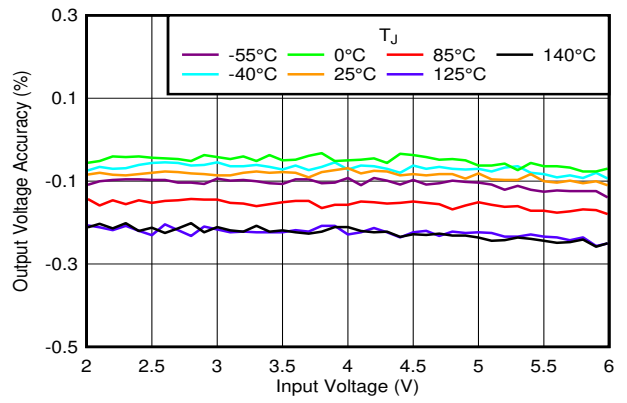
6-26. Output Accuracy vs V_{IN} and Temperature V_{OUT} = 1.8\text{ V} , I_{OUT} = 1\text{ mA}
