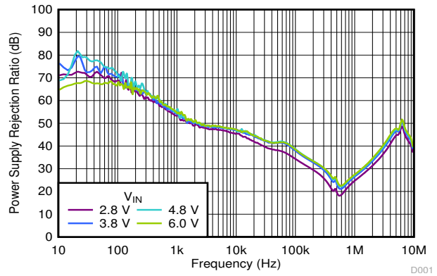
6-44. PSRR vs Frequency and V_{IN}
