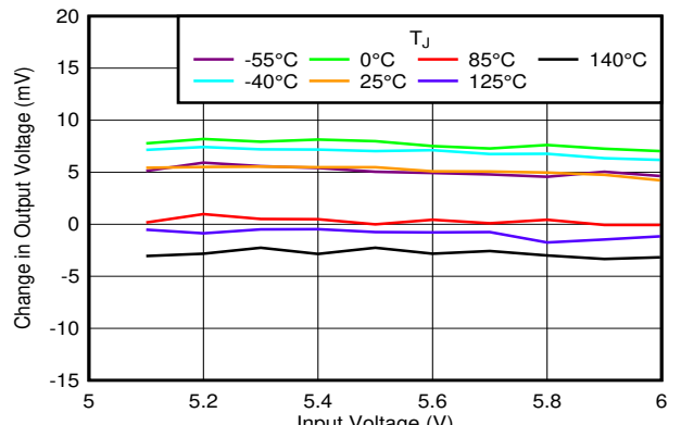
6-28. Line Regulation vs V_{IN} and Temperature V_{OUT} = 5.0\text{ V} , I_{OUT} = 1\text{ mA}
