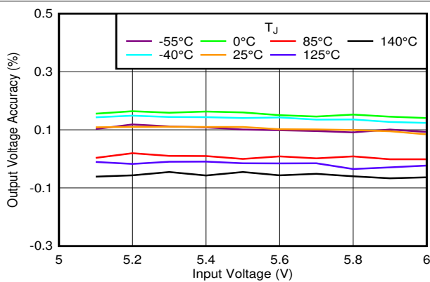
6-29. Output Accuracy vs V_{IN} and Temperature V_{OUT} = 5.0\text{ V} , I_{OUT} = 1\text{ mA}
