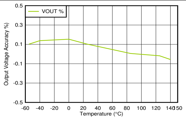
6-30. Output Accuracy vs Temperature V_{OUT} = 5.0\text{ V} , I_{OUT} = 1\text{ mA}
