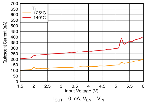
6-2. I_Q vs V_{IN} and Temperature
