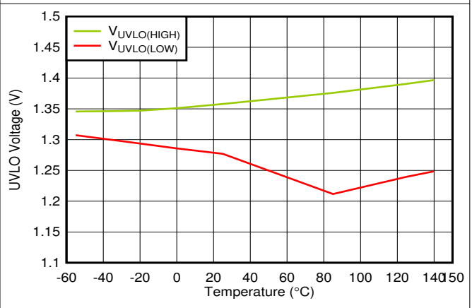
6-40. UVLO Rising and Falling Threshold vs Temperature
