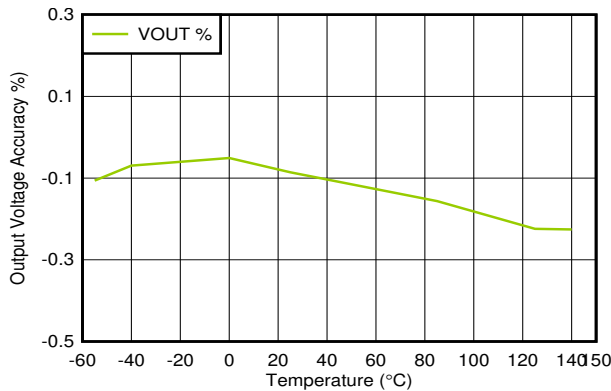
6-27. Output Accuracy vs Temperature V_{OUT} = 1.8\text{ V} , I_{OUT} = 1\text{ mA}
