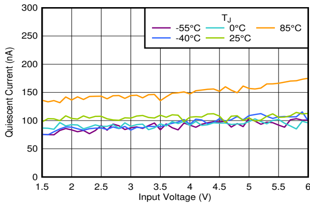
6-1. I_Q vs V_{IN} and Temperature
