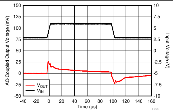
6-24. V_{IN} Transient From 2.8 V to 6.0 V
