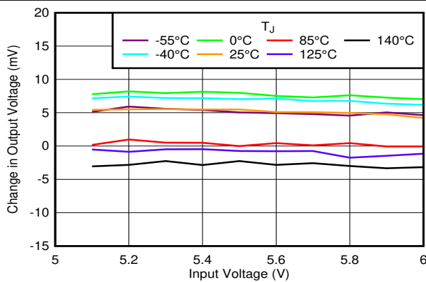
6-27. Output Accuracy vs V_{IN} and Temperature
