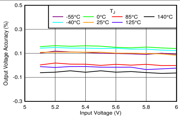
6-30. Output Accuracy vs V_{IN} and Temperature
