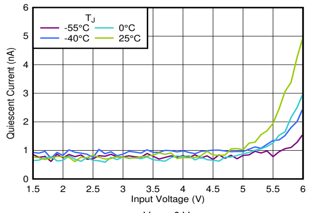
Figure 6-10. I_{SHDN} vs V_{IN} and Temperature
