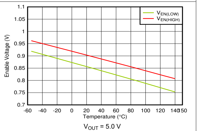
6-40. EN High and Low Threshold vs Temperature
