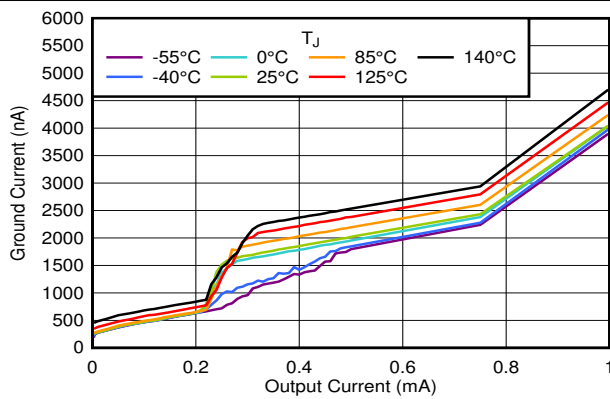
6-5. I_Q vs I_{OUT} and Temperature Up to 1 mA
