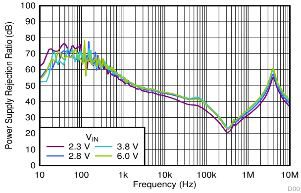
V_{OUT} = 1.8\text{ V} , I_{OUT} = 10\text{ mA} , C_{OUT} = 1\text{ }\mu\text{F} 6-45. PSRR vs Frequency and V_{IN}
