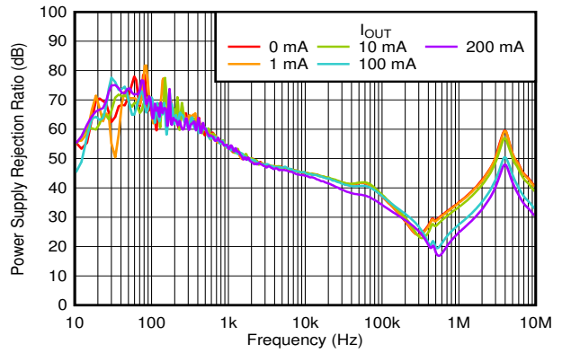
V_{IN} = 2.8\text{ V} , V_{OUT} = 1.8\text{ V} , C_{OUT} = 1\text{ }\mu\text{F} 6-44. PSRR vs Frequency and I_{OUT}
