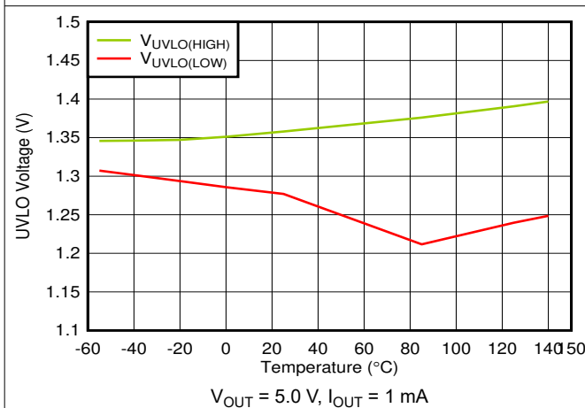
6-41. UVLO Rising and Falling Threshold vs Temperature
