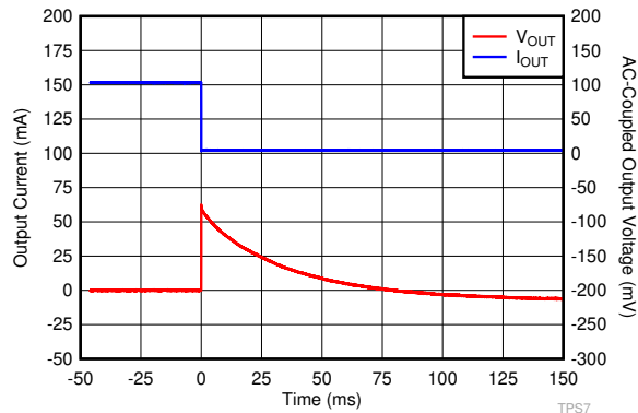
6-19. I_{OUT} Transient From 100 mA to 0 mA
