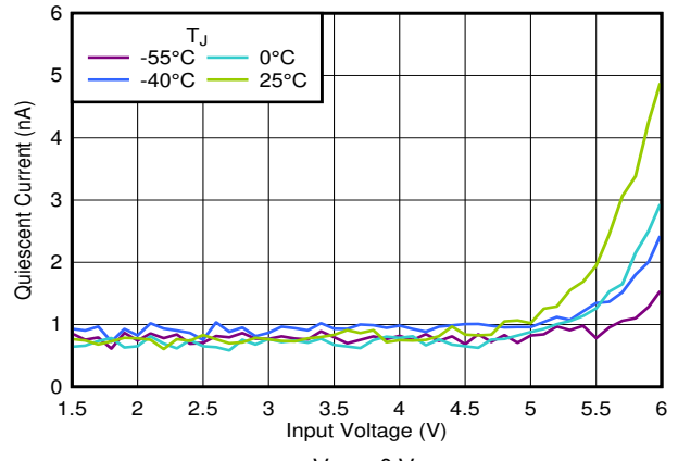
Figure 6-10. I_{SHDN} vs V_{IN} and Temperature
