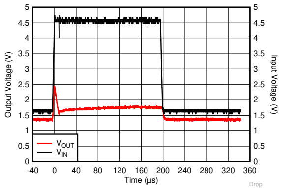
6-25. V_{IN} Transient From 1.5 V to 4.5 V
