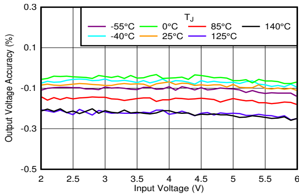
6-27. Output Accuracy vs V_{IN} and Temperature
