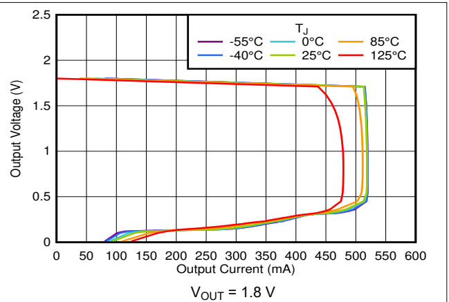
6-38. Foldback Current Limit vs I_{OUT} and Temperature
