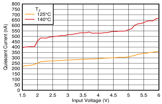
6-2. I_Q vs V_{IN} and Temperature
