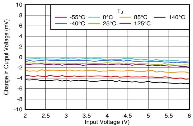
6-26. Line Regulation vs V_{IN} and Temperature
