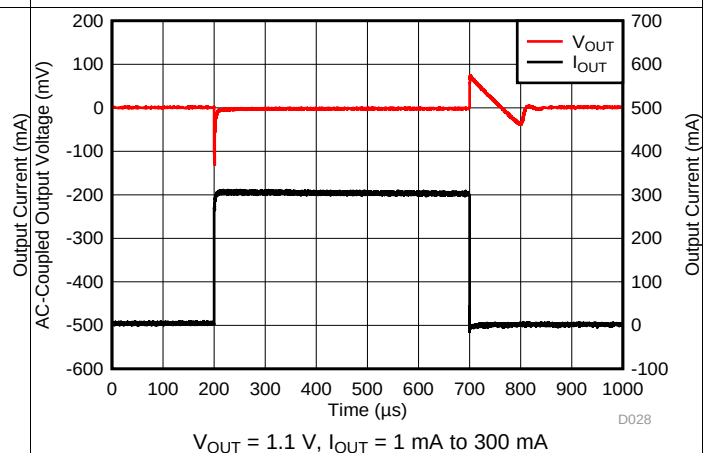
FIG 12. I_{OUT} Transient
