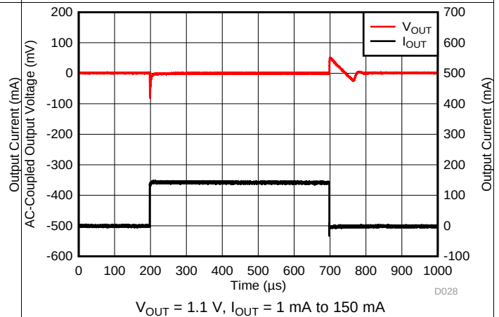
FIG 10. I_{OUT} Transient
