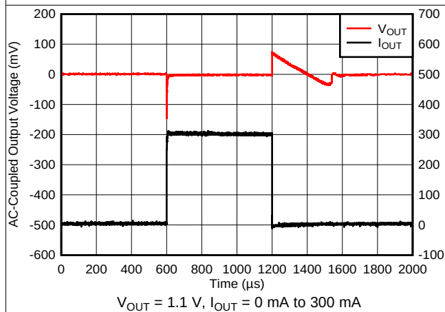
FIG 11. I_{OUT} Transient
