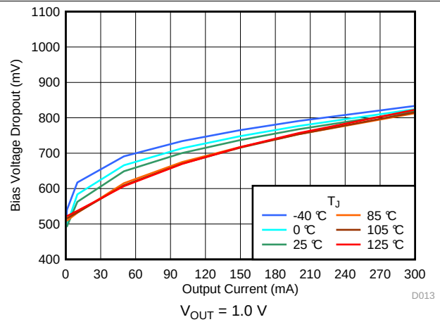
FIG 8. Dropout vs V_{BIAS} and Temperature
