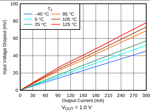
FIG 7. Dropout vs I_{OUT} and Temperature, DSE Package
