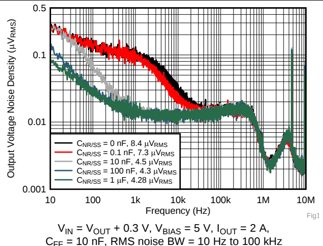
Fig 12. Output Noise vs Frequency and C_{NR/SS}
