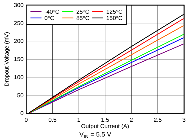
FIG 24. Dropout Voltage vs Output Current (High V_{IN} )
