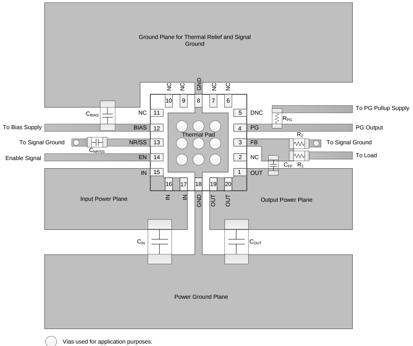
FIG 50. Example Layout
