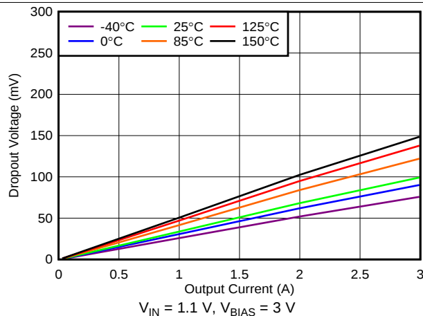
FIG 23. Dropout Voltage vs Output Current With Bias
