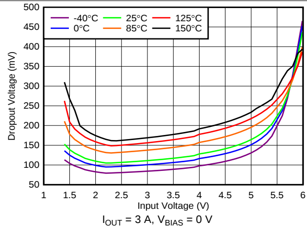
FIG 20. Dropout Voltage vs Input Voltage Without Bias
