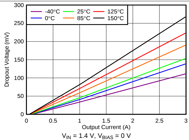
FIG 22. Dropout Voltage vs Output Current Without Bias
