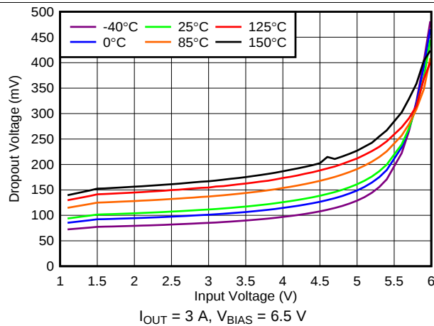
FIG 21. Dropout Voltage vs Input Voltage With Bias
