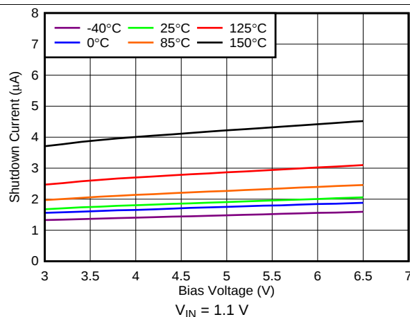
FIG 30. Shutdown Current vs Bias Voltage
