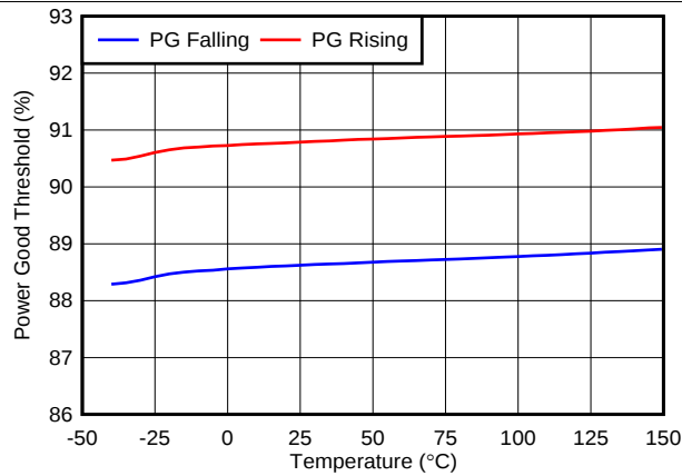
37. PG Threshold vs Temperature
