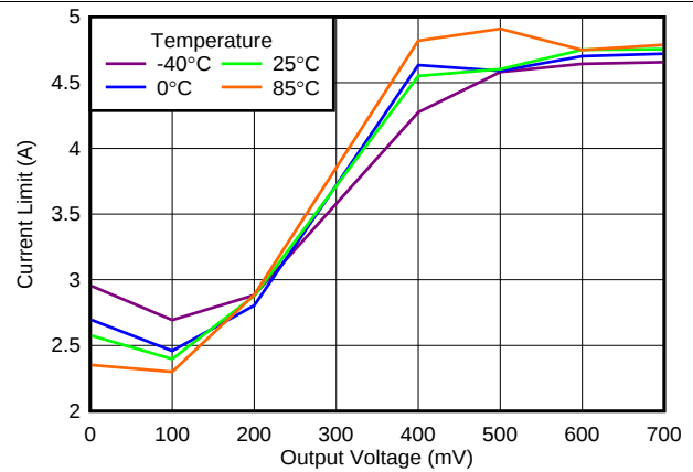
38. Foldback Current Limit vs Temperature
