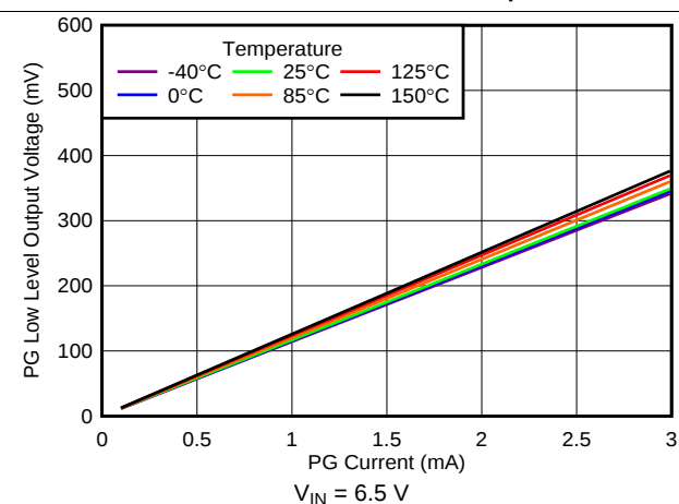
Figure 36. PG Voltage vs PG Current Sink
