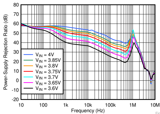
7-4. PSRR vs Frequency and V_{IN}
