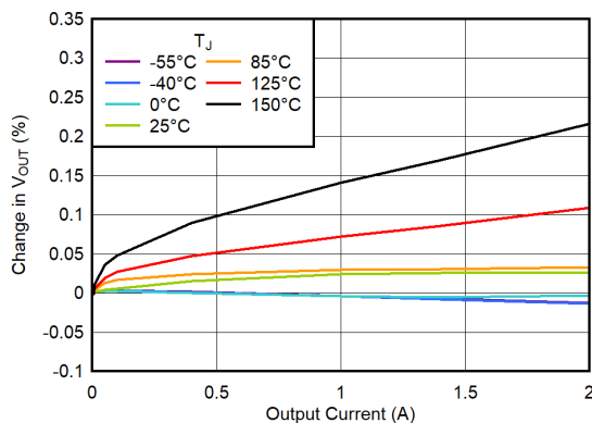
7-51. Load Regulation
