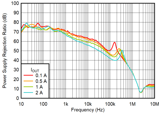
7-43. PSRR vs Frequency and I_{OUT}
