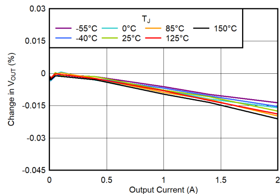
7-52. Load Regulation (3.3-V Output)
