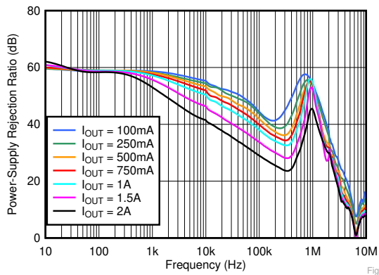
7-1. PSRR vs Frequency and I_{OUT}
