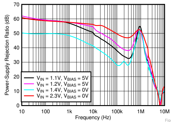
7-2. PSRR vs Frequency and V_{IN} With BIAS
