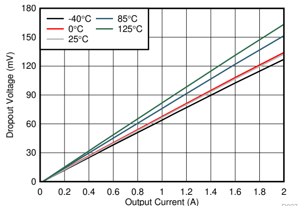
7-48. Dropout Voltage vs Output Current Without BIAS
