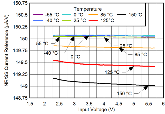
6-44. I_{NR/SS} vs V_{IN} and Temperature for V_{OUT} = 1.8\text{ V}
