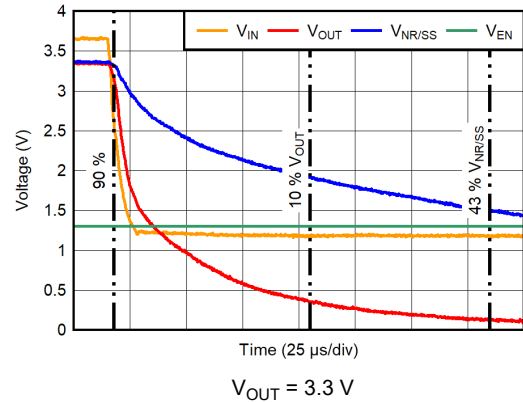
6-26. Shutdown Waveform for UVLO(I_{IN})
