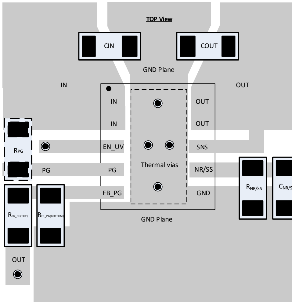
8-33. Example Layout
