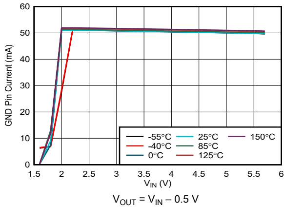
6-57. GND Pin Current vs V_{IN} and Temperature for I_{OUT} = 2\text{ A}
