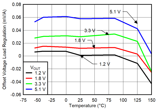
6-35. V_{OS} Load Regulation
