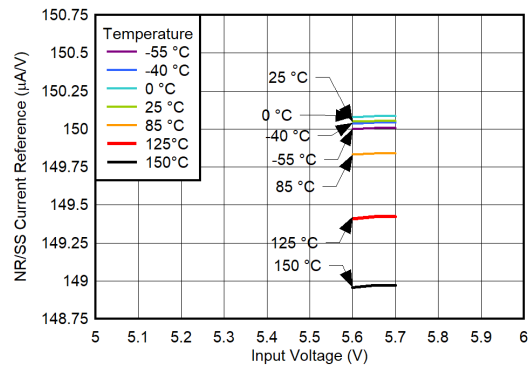
6-48. I_{NR/SS} vs V_{IN} and Temperature for V_{OUT} = 5.1\text{ V}
