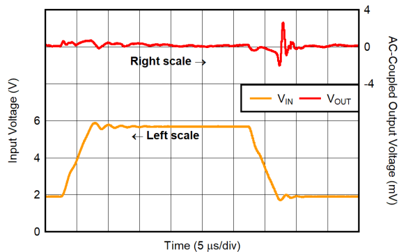
6-24. Line Transient Response for V_{OUT} = 1.2\text{ V} , I_{OUT} = 2\text{ A}
