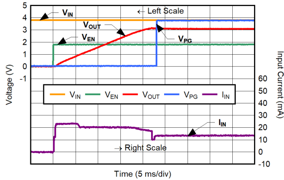
6-31. Inrush Current for C_{NR/SS} = 10\text{ }\mu\text{F}
