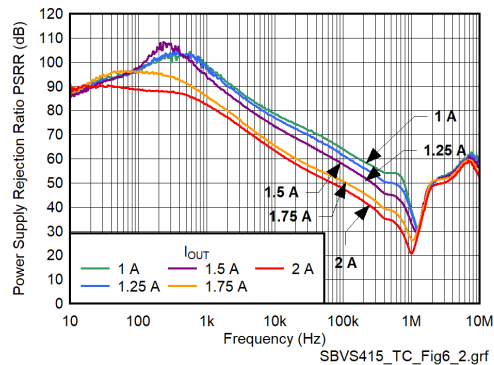
6-2. PSRR vs Frequency and I_{OUT} for V_{OUT} = 1.8\text{ V}
