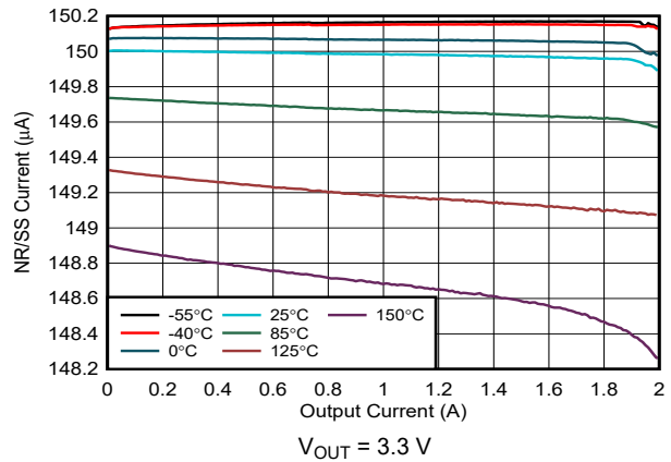
6-40. I_{NR/SS} vs I_{OUT} and Temperature for V_{IN} = 3.8\text{ V}
