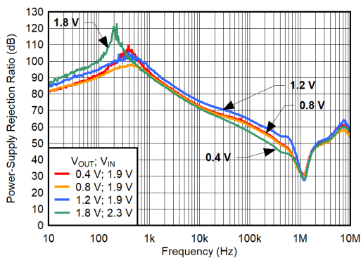
6-5. PSRR vs Frequency and Input Pairs
