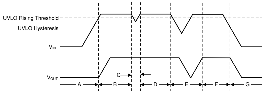
☒ 8-7. Typical UVLO Operation
