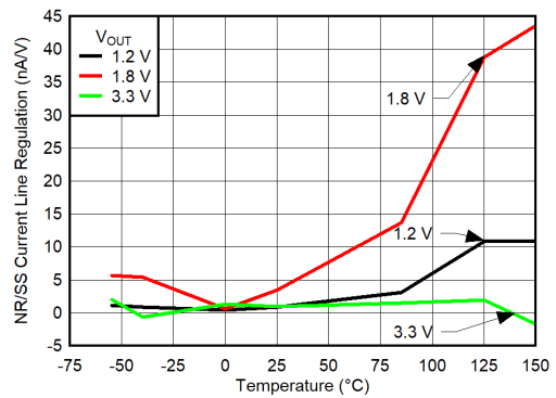
6-36. I_{NR/SS} Line Regulation
