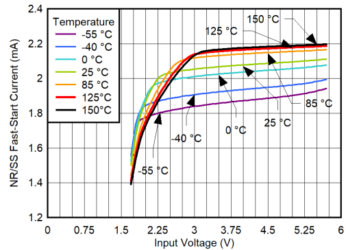
6-52. I_{NR/SS} Fast-Start vs V_{IN} and Temperature
