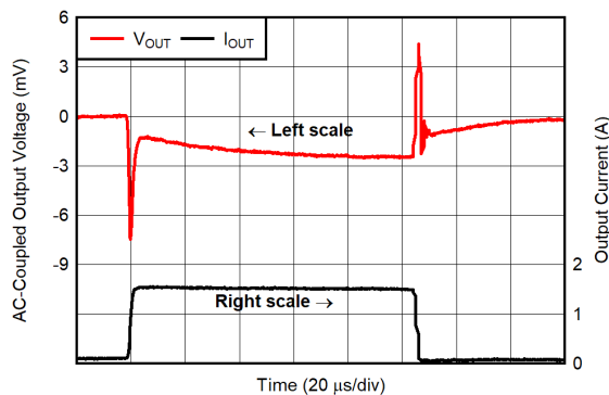
6-17. Load Transient Response for V_{OUT} = 1.2\text{ V} , I_{OUT} = 100\text{ mA} to 1.5\text{ A}
