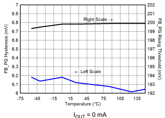
6-66. V_{FB\_PG} Hysteresis and Threshold vs Temperature
