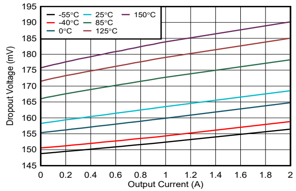
6-32. Dropout Voltage vs I_{OUT} for V_{OUT} = 1.8\text{ V}
