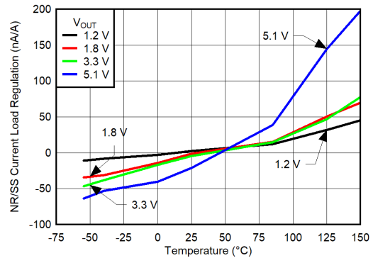
6-34. I_{NR/SS} Load Regulation
