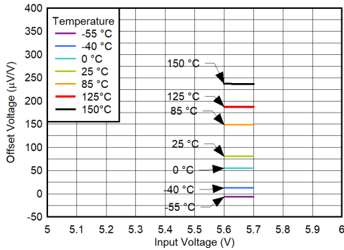
6-49. V_{OS} vs V_{IN} and Temperature for V_{OUT} = 5.1\text{ V}
