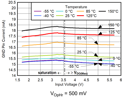
6-55. GND Pin Current vs V_{IN} and Temperature for I_{OUT} = 1\text{ mA}
