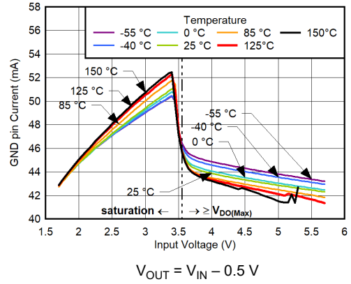
6-56. GND Pin Current vs V_{IN} and Temperature for I_{OUT} = 1\text{ A}
