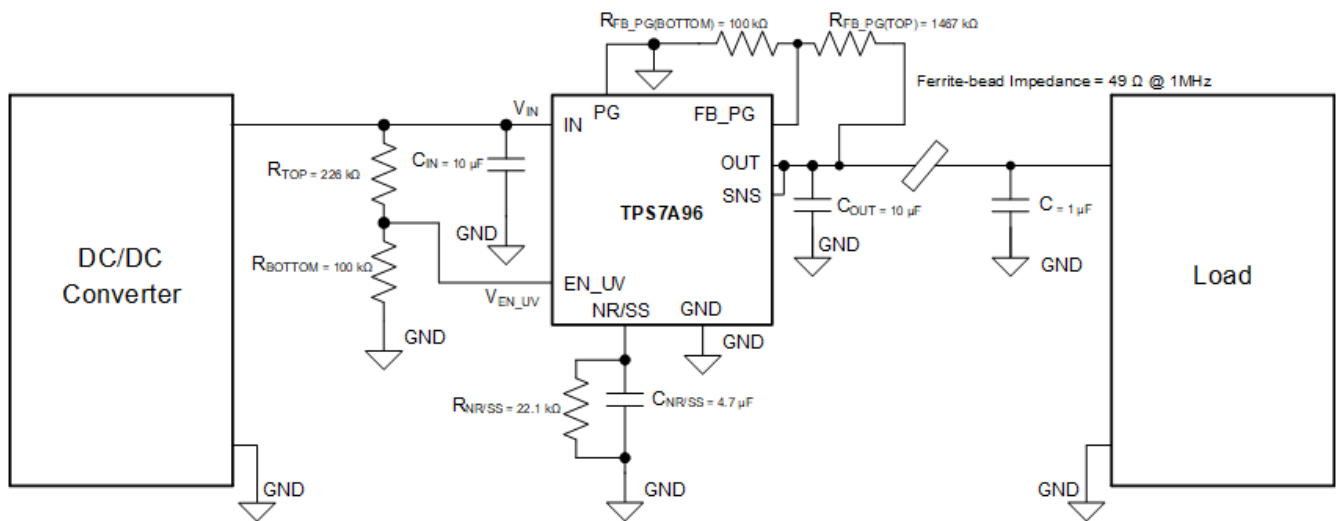
8-27. Typical Application Circuit With Added Pi-Filter
