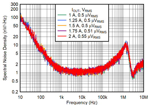
6-15. Output Voltage Noise Density vs Frequency for I_{OUT} and V_{OUT} = 5.0\text{ V}
