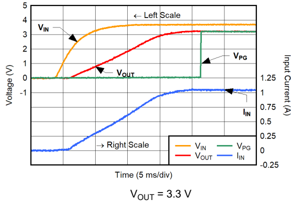
6-25. Start-Up Waveform for I_{OUT} = 1\text{ A}
