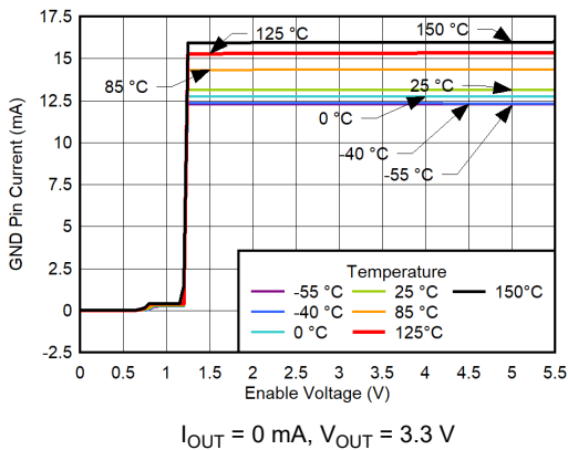
6-59. GND Pin Current vs V_{EN} and Temperature for V_{IN} = 5.7\text{ V}
