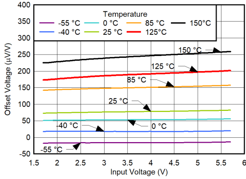
6-43. V_{OS} vs V_{IN} and Temperature for V_{OUT} = 1.2\text{ V}
