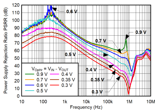
6-6. PSRR vs Frequency for Operating Headroom ( V_{OPHR} )
