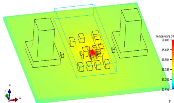
☒ 8-25. TPS7A96EVM-106 Device Thermal Gradient
