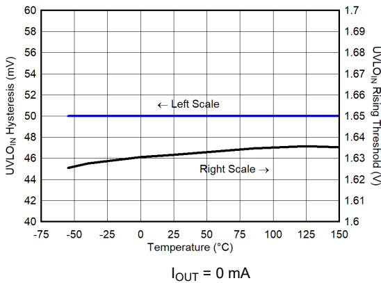
6-63. UVLO_{IN} vs Temperature
