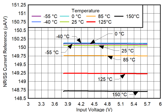
8-11. I_{NR/SS} Reference vs Input Voltage and Temperature for V_{OUT} = 3.3 V
