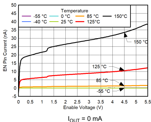
6-65. EN Pin Current vs V_{EN} and Temperature for V_{IN} = 5.7\text{ V}
