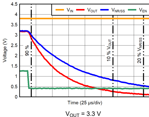
6-27. Shutdown Waveform With EN
