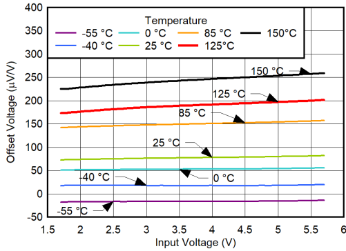
6-45. V_{OS} vs V_{IN} and Temperature for V_{OUT} = 1.8\text{ V}
