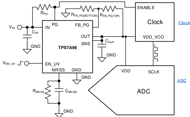
図 8-15. Typical Circuit
