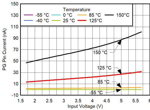
6-69. PG Pin Current vs V_{IN} and Temperature
