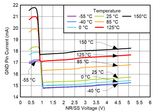
6-54. GND Pin Current vs V_{NR/SS} and Temperature
