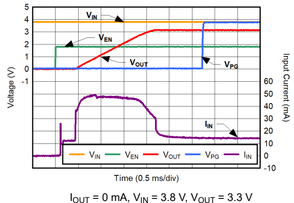
6-28. Inrush Current for C_{NR/SS} = 1.0\text{ }\mu\text{F}
