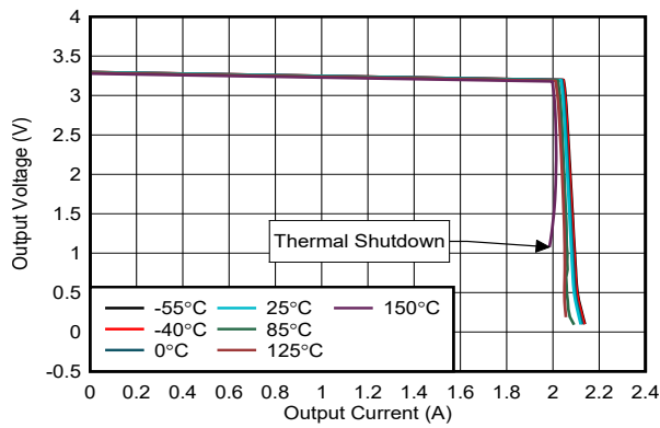
6-61. 80% Current Limit vs Temperature for V_{OUT} = 3.3\text{ V}
