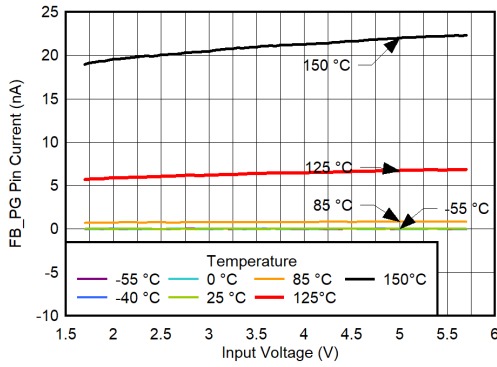
6-67. FB_PG Pin Current vs V_{IN} and Temperature
