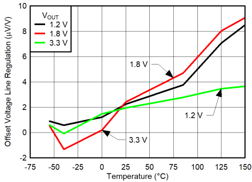
6-37. V_{OS} Line Regulation
