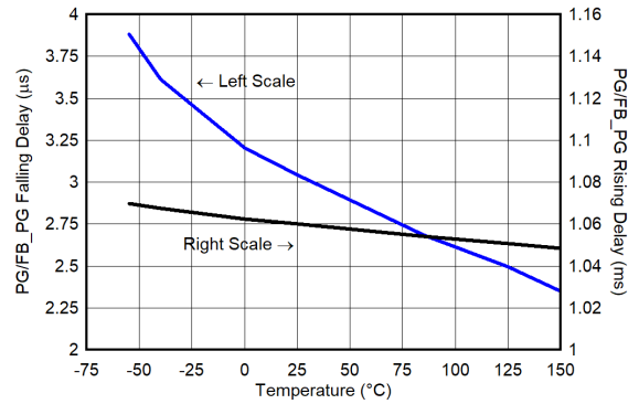
6-70. FB_PG Pin to PG Pin Rising and Falling Delay vs Temperature
