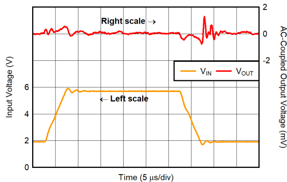
6-23. Line Transient Response for V_{OUT} = 1.2\text{ V} , I_{OUT} = 1.5\text{ A}
