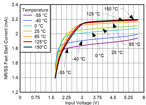
8-12. I_{FAST\_SS} Reference vs Input Voltage and Temperature for V_{OUT} = 3.3 V
