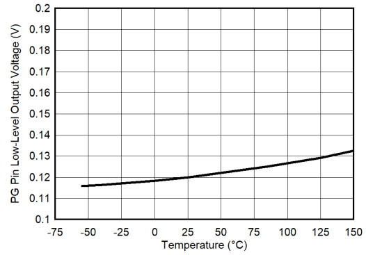
6-68. V_{PG} Low-Level Output Voltage vs Temperature
