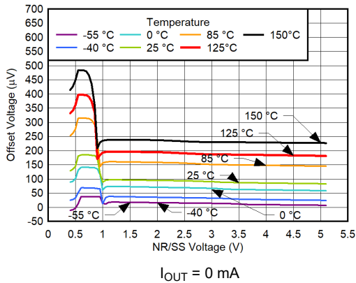
6-39. V_{OS} vs V_{NR/SS} and Temperature for I_{OUT} = 0\text{ mA}
