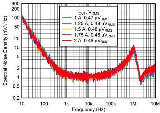
6-13. Output Voltage Noise Density vs Frequency for I_{OUT} and V_{OUT} = 1.8\text{ V}
