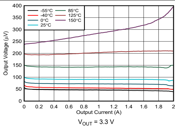
6-41. V_{OS} vs I_{OUT} and Temperature for V_{IN} = 3.8\text{ V}
