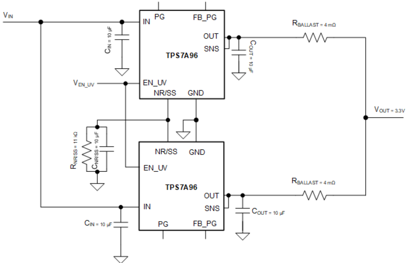
8-16. Paralleling Multiple TPS7A96 Devices
