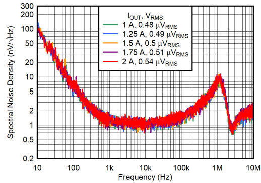
6-14. Output Voltage Noise Density vs Frequency for I_{OUT} and V_{OUT} = 3.3\text{ V}
