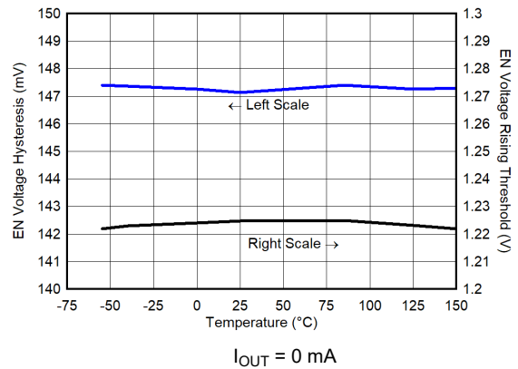
6-64. V_{EN} Hysteresis and Threshold vs Temperature
