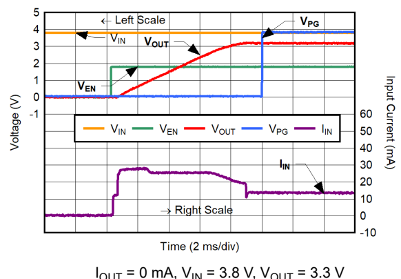
6-30. Inrush Current for C_{NR/SS} = 4.7\text{ }\mu\text{F}
