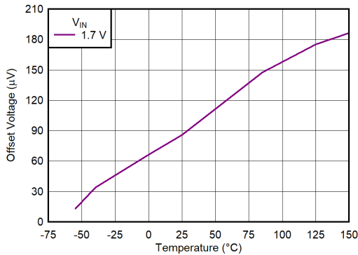
6-51. V_{OS} vs Temperature for V_{IN\_Min} , V_{OpHr} = 0.2\text{ V}
