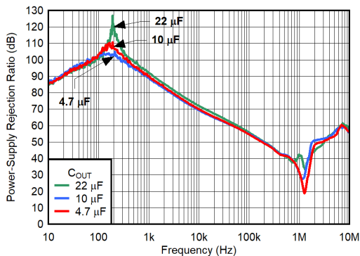
6-11. PSRR vs Frequency and C_{OUT}
