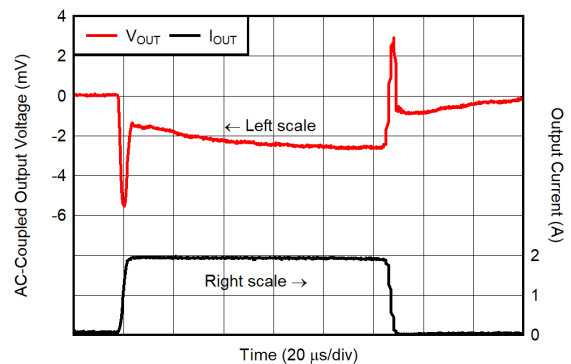
6-18. Load Transient Response for V_{OUT} = 1.2\text{ V} , I_{OUT} = 100\text{ mA} to 2\text{ A}
