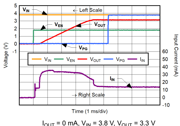
6-29. Inrush Current for C_{NR/SS} = 2.2\text{ }\mu\text{F}
