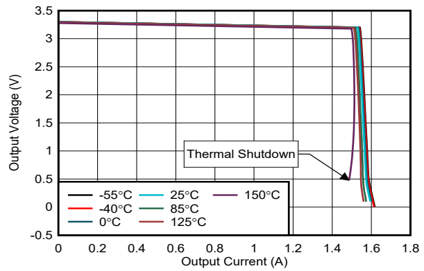
6-62. 60% Current Limit vs Temperature for V_{OUT} = 3.3\text{ V}
