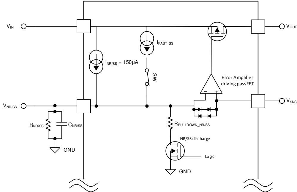
8-10. Simplified Soft-Start Circuit
