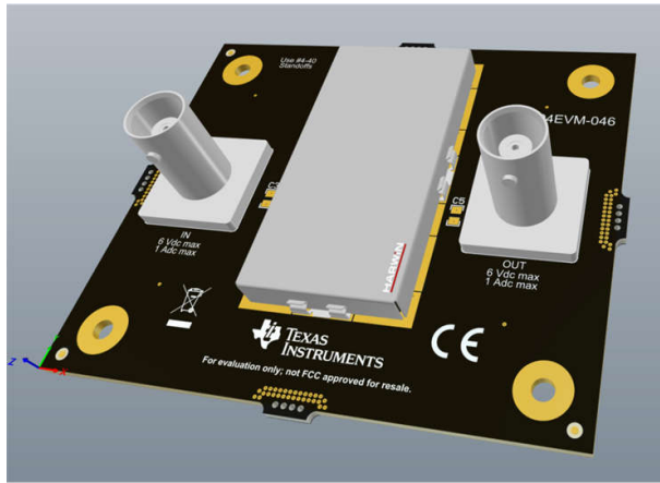
☒ 8-23. TPS7A96EVM-106 3D View
