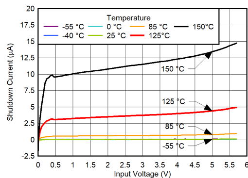
6-72. Shutdown Current vs V_{IN} and Temperature
