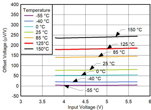
6-47. V_{OS} vs V_{IN} and Temperature for V_{OUT} = 3.3\text{ V}
