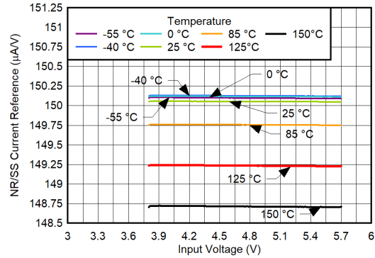
6-46. I_{NR/SS} vs V_{IN} and Temperature for V_{OUT} = 3.3\text{ V}
