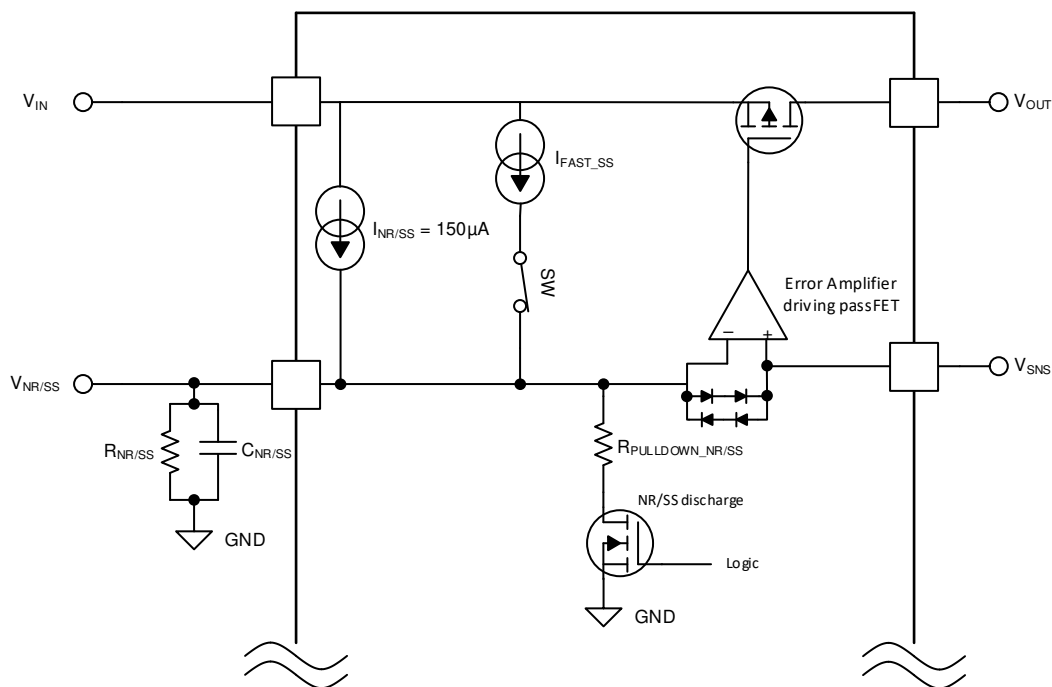
Figure 7-1. Simplified Regulation Circuit
