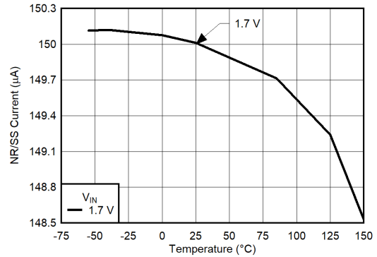
6-50. I_{NR/SS} vs Temperature for V_{IN\_Min} , V_{OpHr} = 0.2\text{ V}
