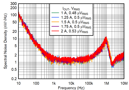
6-12. Output Voltage Noise Density vs Frequency for I_{OUT} and V_{OUT} = 1.2\text{ V}
