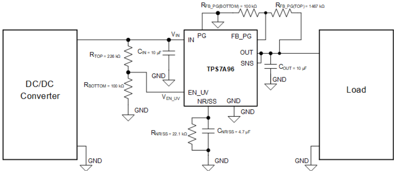
8-26. Typical Application Circuit
