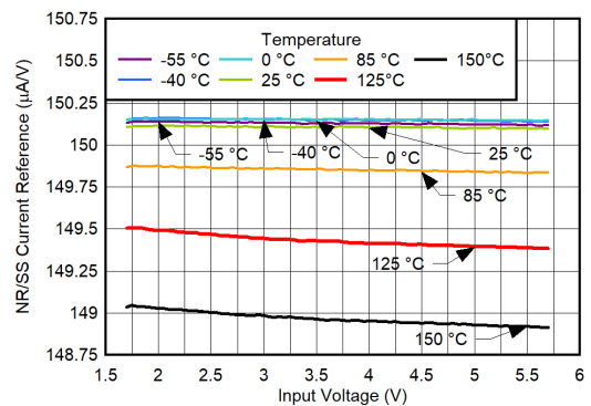
6-42. I_{NR/SS} vs V_{IN} and Temperature for V_{OUT} = 1.2\text{ V}
